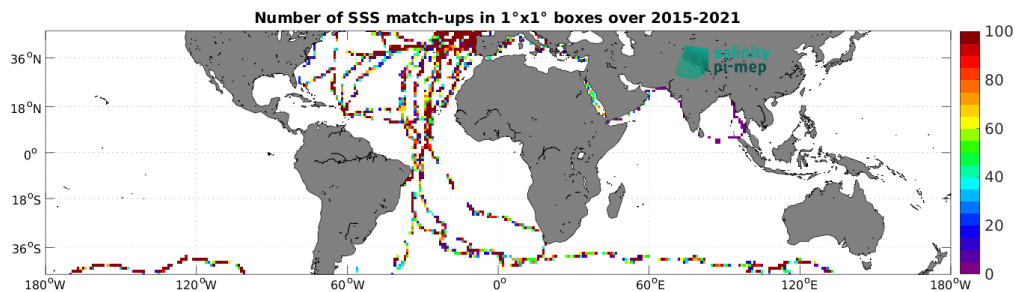
Figure 4: Number of SSS match-ups between TSG (GOSUD-Sailing-ship) SSS and the SMAP SSS L2 v5.0 (JPL) SSS product for the Mid-Low Latitudes 45N-45S Pi-MEP region over 1^\circ \times 1^\circ boxes and for the full satellite product period.
