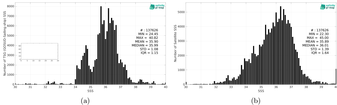
Figure 2: Histograms of SSS from TSG (GOSUD-Sailing-ship) (a) and SMAP SSS L2 v5.0 (JPL) (b) considering all match-up pairs per bins of 0.1 over the Mid-Low Latitudes 45N-45S Pi-MEP region and for the full satellite product period.
