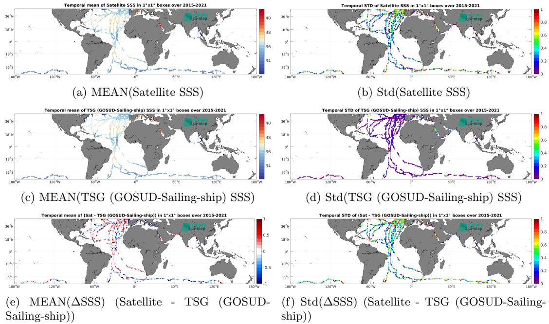
Figure 6: Temporal mean (left) and Std (right) of SSS from SMAP SSS L2 v5.0 (JPL) (top), TSG (GOSUD-Sailing-ship) (middle), and of \Delta SSS (Satellite - TSG (GOSUD-Sailing-ship)). Only match-up pairs are used to generate these maps.
