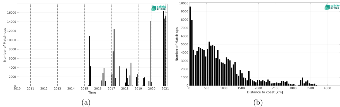
Figure 1: Number of match-ups between TSG (GOSUD-Sailing-ship) and SMAP SSS L2 v5.0 (JPL) SSS as a function of time (a) and as function of the distance to coast (b) over the Mid-Low Latitudes 45N-45S Pi-MEP region and for the full satellite product period.
