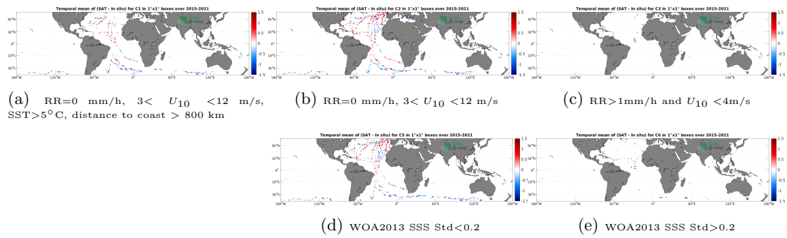
Figure 12: Temporal mean gridded over spatial boxes of size 1^\circ \times 1^\circ of \Delta SSS (SMAP SSS L2 v5.0 (JPL) - TSG (GOSUD-Sailing-ship)) for 5 different subdatasets corresponding to:RR=0 mm/h, 3 < U_{10} < 12 m/s, SST >5^\circ C, distance to coast > 800 km (a), RR=0 mm/h, 3 < U_{10} < 12 m/s (b), RR >1 mm/h and U_{10} < 4 m/s (c), WOA2013 SSS Std <0.2 (d), WOA2013 SSS Std >0.2 (e).
