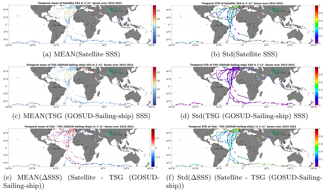
Figure 6: Temporal mean (left) and Std (right) of SSS from SMAP SSS L2 v5.0 (JPL) (top), TSG (GOSUD-Sailing-ship) (middle), and of \Delta SSS (Satellite - TSG (GOSUD-Sailing-ship)). Only match-up pairs are used to generate these maps.
