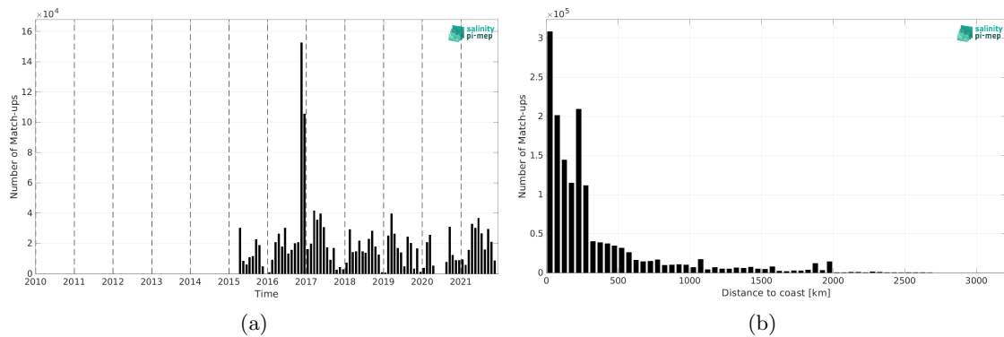
Figure 2: Number of match-ups between TSG (GOSUD-Research-vessel) and SMAP SSS L2 v5.0 (JPL) SSS as a function of time (a) and as function of the distance to coast (b) over the Mid-Low Latitudes 45N-45S Pi-MEP region and for the full satellite product period.
