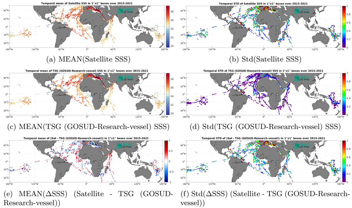
Figure 7: Temporal mean (left) and Std (right) of SSS from SMAP SSS L2 v5.0 (JPL) (top), TSG (GOSUD-Research-vessel) (middle), and of \Delta SSS (Satellite - TSG (GOSUD-Research-vessel)). Only match-up pairs are used to generate these maps.
