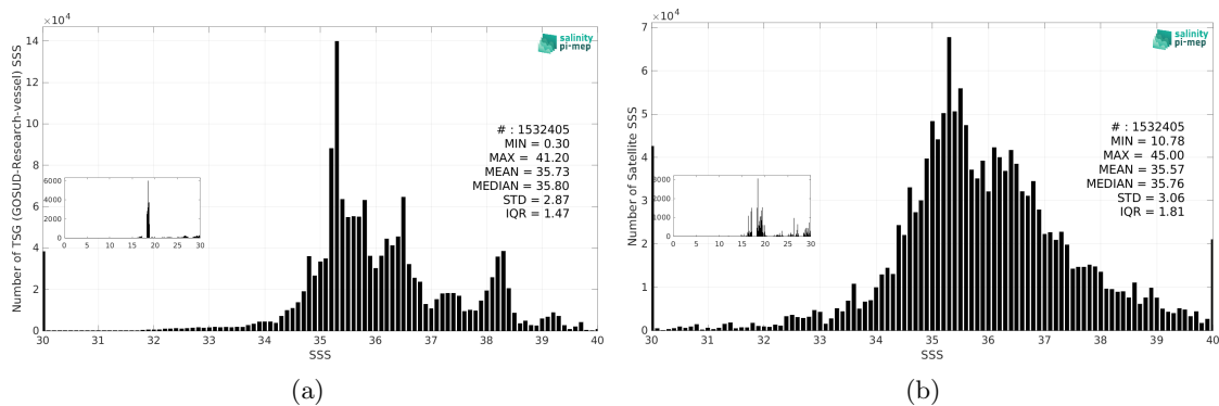
Figure 3: Histograms of SSS from TSG (GOSUD-Research-vessel) (a) and SMAP SSS L2 v5.0 (JPL) (b) considering all match-up pairs per bins of 0.1 over the Mid-Low Latitudes 45N-45S Pi-MEP region and for the full satellite product period.
