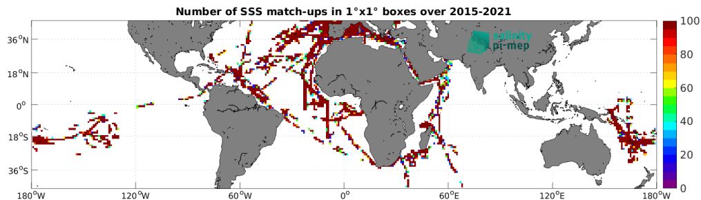
Figure 5: Number of SSS match-ups between TSG (GOSUD-Research-vessel) SSS and the SMAP SSS L2 v5.0 (JPL) SSS product for the Mid-Low Latitudes 45N-45S Pi-MEP region over 1^\circ \times 1^\circ boxes and for the full satellite product period.
