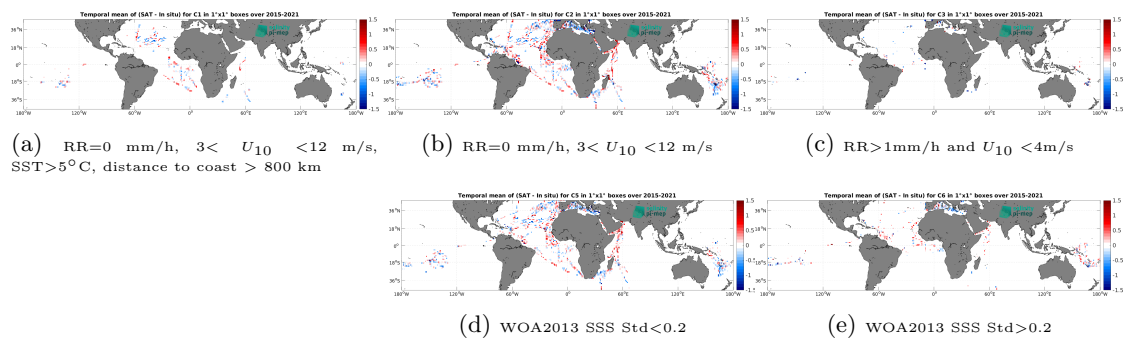
Figure 14: Temporal mean gridded over spatial boxes of size 1^\circ \times 1^\circ of \Delta SSS (SMAP SSS L2 v5.0 (JPL) - TSG (GOSUD-Research-vessel)) for 5 different subdatasets corresponding to: RR=0 mm/h, 3 < U_{10} < 12 m/s, SST > 5°C, distance to coast > 800 km (a), RR=0 mm/h, 3 < U_{10} < 12 m/s (b), RR > 1mm/h and U_{10} < 4 m/s (c), WOA2013 SSS Std < 0.2 (d), WOA2013 SSS Std > 0.2 (e).
