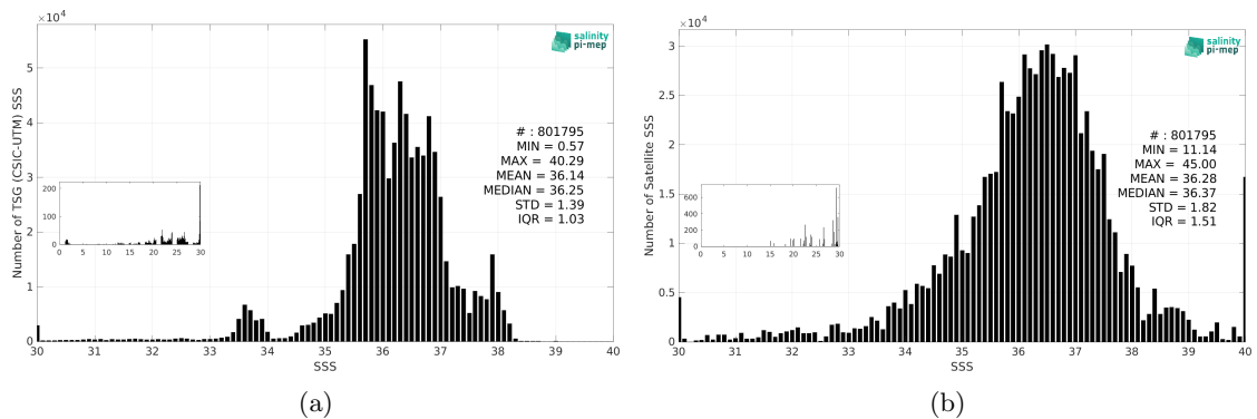
Figure 3: Histograms of SSS from TSG (CSIC-UTM) (a) and SMAP SSS L2 v5.0 (JPL) (b) considering all match-up pairs per bins of 0.1 over the Mid-Low Latitudes 45N-45S Pi-MEP region and for the full satellite product period.
