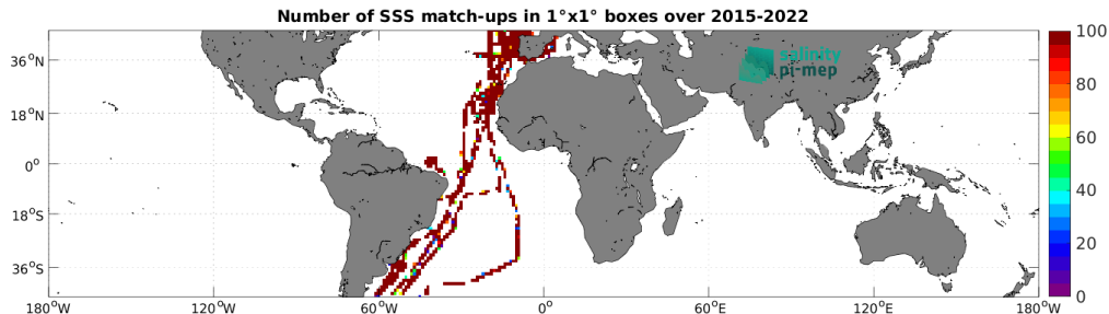
Figure 5: Number of SSS match-ups between TSG (CSIC-UTM) SSS and the SMAP SSS L2 v5.0 (JPL) SSS product for the Mid-Low Latitudes 45N-45S Pi-MEP region over 1^\circ \times 1^\circ boxes and for the full satellite product period.
