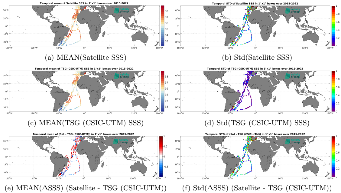
Figure 7: Temporal mean (left) and Std (right) of SSS from SMAP SSS L2 v5.0 (JPL) (top), TSG (CSIC-UTM) (middle), and of \Delta SSS (Satellite - TSG (CSIC-UTM)). Only match-up pairs are used to generate these maps.
