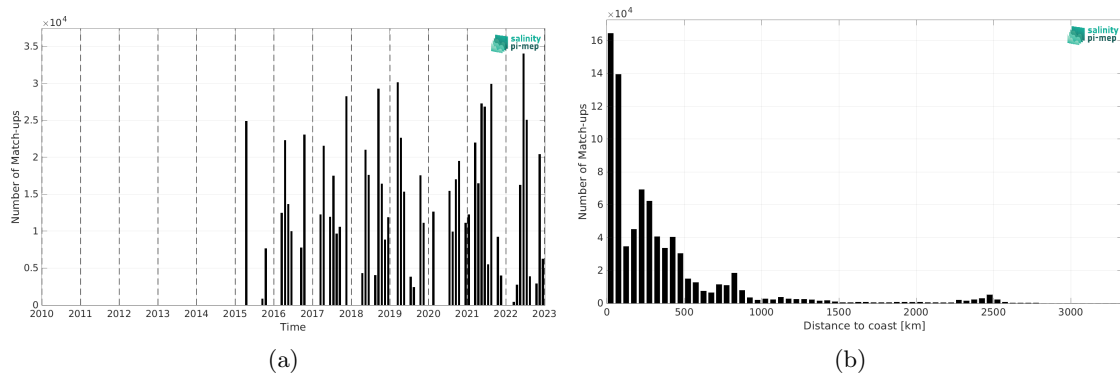
Figure 2: Number of match-ups between TSG (CSIC-UTM) and SMAP SSS L2 v5.0 (JPL) SSS as a function of time (a) and as function of the distance to coast (b) over the Mid-Low Latitudes 45N-45S Pi-MEP region and for the full satellite product period.
