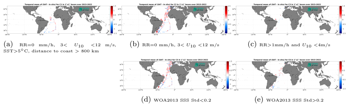
Figure 14: Temporal mean gridded over spatial boxes of size 1^\circ \times 1^\circ of \Delta\text{SSS} (SMAP SSS L2 v5.0 (JPL) - TSG (CSIC-UTM)) for 5 different subdatasets corresponding to: RR=0 mm/h, 3 < U_{10} < 12 m/s, SST > 5°C, distance to coast > 800 km (a), RR=0 mm/h, 3 < U_{10} < 12 m/s (b), RR > 1mm/h and U_{10} < 4 m/s (c), WOA2013 SSS Std < 0.2 (d), WOA2013 SSS Std > 0.2 (e).
