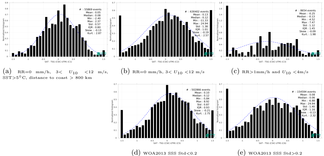
Figure 13: Normalized histogram of \Delta SSS (SMAP SSS L2 v5.0 (JPL) - TSG (CSIC-UTM)) for 5 different subdatasets corresponding to: RR=0 mm/h, 3 < U_{10} < 12 m/s, SST>5°C, distance to coast > 800 km (a), RR=0 mm/h, 3 < U_{10} < 12 m/s (b), RR>1mm/h and U_{10} < 4 m/s (c), WOA2013 SSS Std<0.2 (d), WOA2013 SSS Std>0.2 (e).
