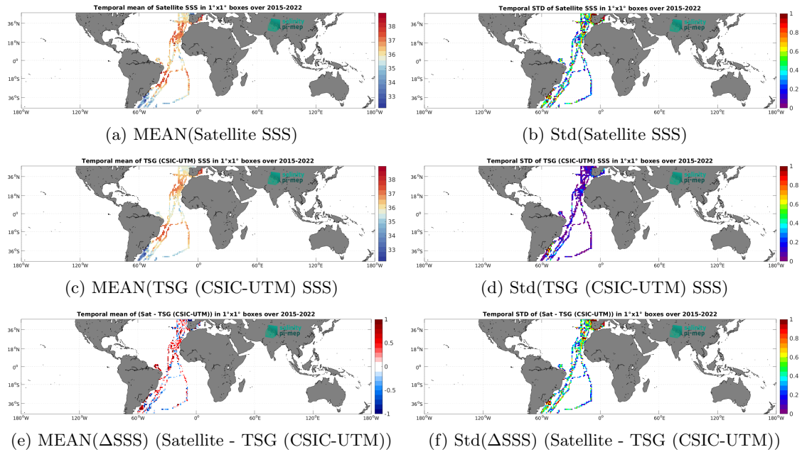
Figure 6: Temporal mean (left) and Std (right) of SSS from SMAP SSS L2 v5.0 (JPL) (top), TSG (CSIC-UTM) (middle), and of \Delta SSS (Satellite - TSG (CSIC-UTM)). Only match-up pairs are used to generate these maps.
