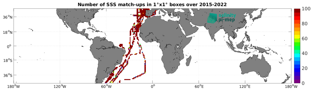
Figure 4: Number of SSS match-ups between TSG (CSIC-UTM) SSS and the SMAP SSS L2 v5.0 (JPL) SSS product for the Mid-Low Latitudes 45N-45S Pi-MEP region over 1^\circ \times 1^\circ boxes and for the full satellite product period.
