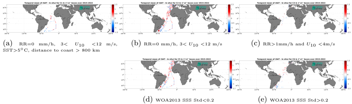
Figure 12: Temporal mean gridded over spatial boxes of size 1^\circ \times 1^\circ of \Delta SSS (SMAP SSS L2 v5.0 (JPL) - TSG (CSIC-UTM)) for 5 different subdatasets corresponding to: RR=0 mm/h, 3 < U_{10} < 12 m/s, SST>5°C, distance to coast > 800 km (a), RR=0 mm/h, 3 < U_{10} < 12 m/s (b), RR>1mm/h and U_{10} < 4 m/s (c), WOA2013 SSS Std<0.2 (d), WOA2013 SSS Std>0.2 (e).
