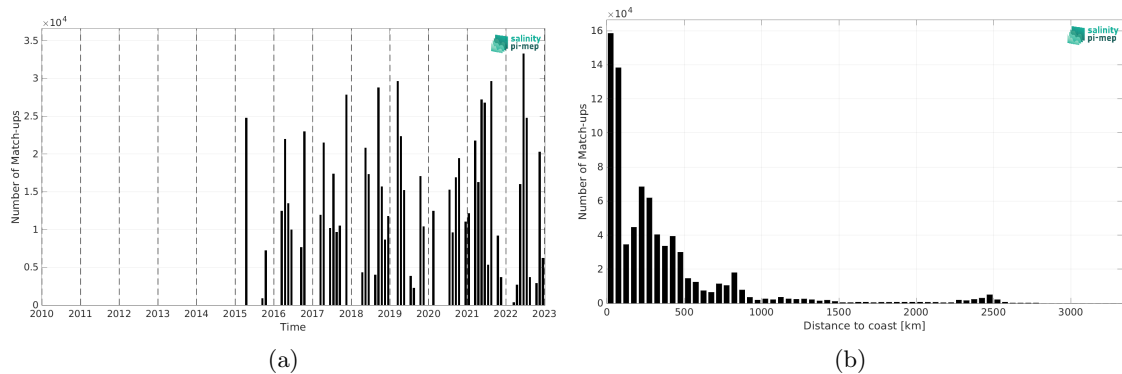
Figure 1: Number of match-ups between TSG (CSIC-UTM) and SMAP SSS L2 v5.0 (JPL) SSS as a function of time (a) and as function of the distance to coast (b) over the Mid-Low Latitudes 45N-45S Pi-MEP region and for the full satellite product period.
