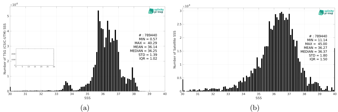
Figure 2: Histograms of SSS from TSG (CSIC-UTM) (a) and SMAP SSS L2 v5.0 (JPL) (b) considering all match-up pairs per bins of 0.1 over the Mid-Low Latitudes 45N-45S Pi-MEP region and for the full satellite product period.
