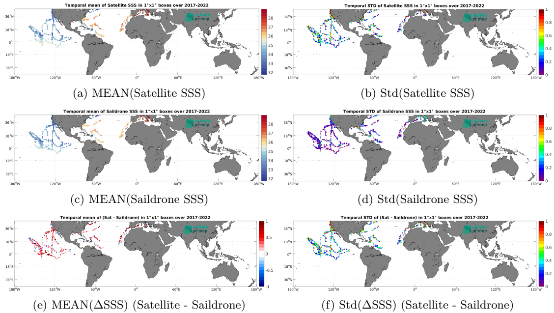
Figure 7: Temporal mean (left) and Std (right) of SSS from SMAP SSS L2 v5.0 (JPL) (top), Saildrone (middle), and of \Delta SSS (Satellite - Saildrone). Only match-up pairs are used to generate these maps.
