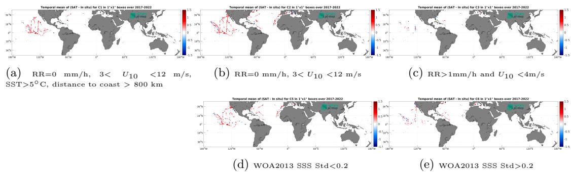
Figure 14: Temporal mean gridded over spatial boxes of size 1^\circ \times 1^\circ of \Delta SSS (SMAP SSS L2 v5.0 (JPL) - Saldrone) for 5 different subdatasets corresponding to: RR=0 mm/h, 3 < U_{10} < 12 m/s, SST > 5°C, distance to coast > 800 km (a), RR=0 mm/h, 3 < U_{10} < 12 m/s (b), RR > 1mm/h and U_{10} < 4 m/s (c), WOA2013 SSS Std < 0.2 (d), WOA2013 SSS Std > 0.2 (e).
