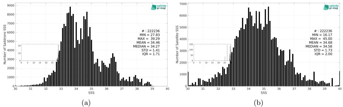
Figure 3: Histograms of SSS from Sairdrone (a) and SMAP SSS L2 v5.0 (JPL) (b) considering all match-up pairs per bins of 0.1 over the Mid-Low Latitudes 45N-45S Pi-MEP region and for the full satellite product period.
