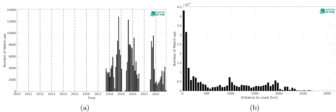
Figure 2: Number of match-ups between Sairdrone and SMAP SSS L2 v5.0 (JPL) SSS as a function of time (a) and as function of the distance to coast (b) over the Mid-Low Latitudes 45N-45S Pi-MEP region and for the full satellite product period.
