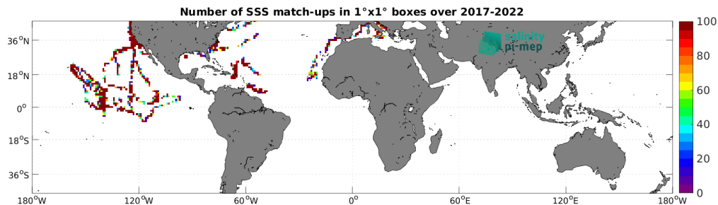
Figure 5: Number of SSS match-ups between Saildrone SSS and the SMAP SSS L2 v5.0 (JPL) SSS product for the Mid-Low Latitudes 45N-45S Pi-MEP region over 1^\circ \times 1^\circ boxes and for the full satellite product period.
