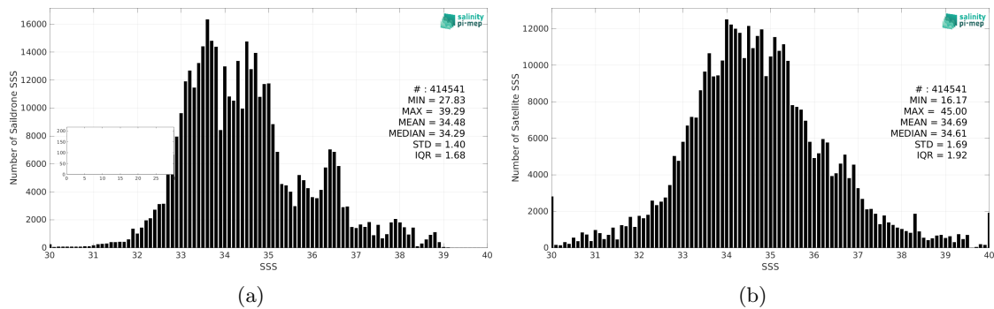
Figure 2: Histograms of SSS from Sairdrone (a) and SMAP SSS L2 v5.0 (JPL) (b) considering all match-up pairs per bins of 0.1 over the Mid-Low Latitudes 45N-45S Pi-MEP region and for the full satellite product period.
