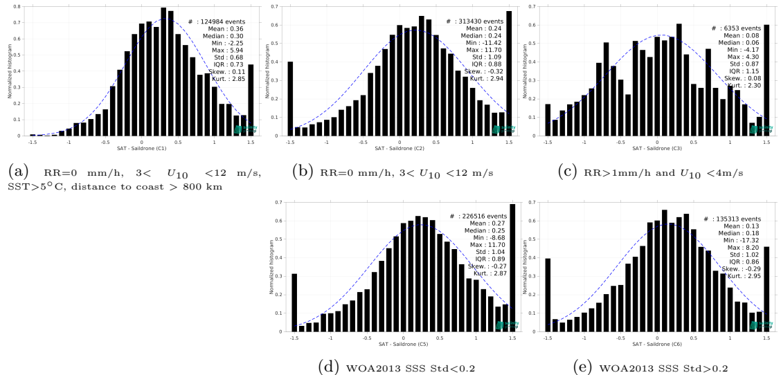
Figure 13: Normalized histogram of \Delta SSS (SMAP SSS L2 v5.0 (JPL) - Saildrone) for 5 different subdatasets corresponding to: RR=0 mm/h, 3 < U_{10} < 12 m/s, SST >5^\circ\text{C} , distance to coast > 800 km (a), RR=0 mm/h, 3 < U_{10} < 12 m/s (b), RR >1 mm/h and U_{10} < 4 m/s (c), WOA2013 SSS Std <0.2 (d), WOA2013 SSS Std >0.2 (e).
