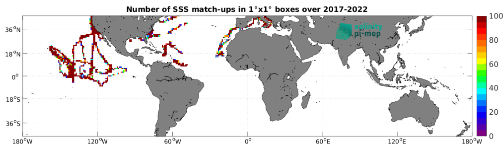
Figure 4: Number of SSS match-ups between Saildrone SSS and the SMAP SSS L2 v5.0 (JPL) SSS product for the Mid-Low Latitudes 45N-45S Pi-MEP region over 1^\circ \times 1^\circ boxes and for the full satellite product period.
