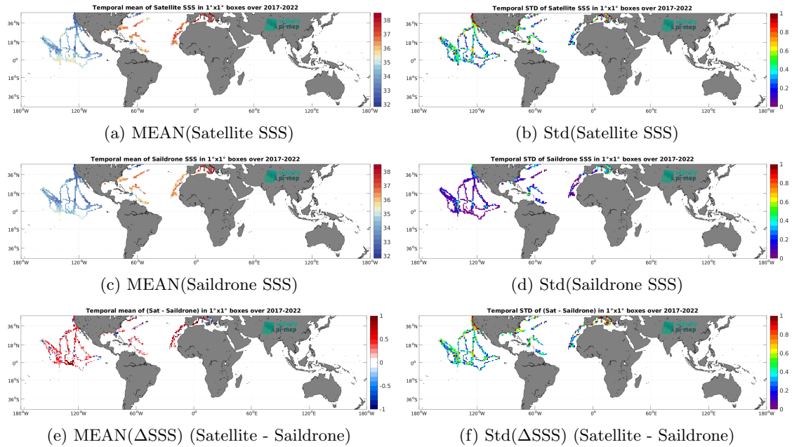
Figure 6: Temporal mean (left) and Std (right) of SSS from SMAP SSS L2 v5.0 (JPL) (top), Saildrone (middle), and of \Delta SSS (Satellite - Saildrone). Only match-up pairs are used to generate these maps.
