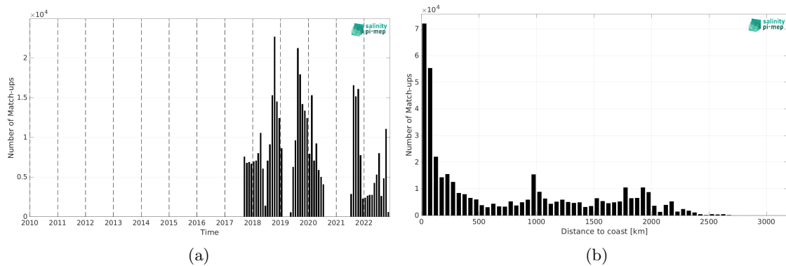
Figure 1: Number of match-ups between Sairdrone and SMAP SSS L2 v5.0 (JPL) SSS as a function of time (a) and as function of the distance to coast (b) over the Mid-Low Latitudes 45N-45S Pi-MEP region and for the full satellite product period.
