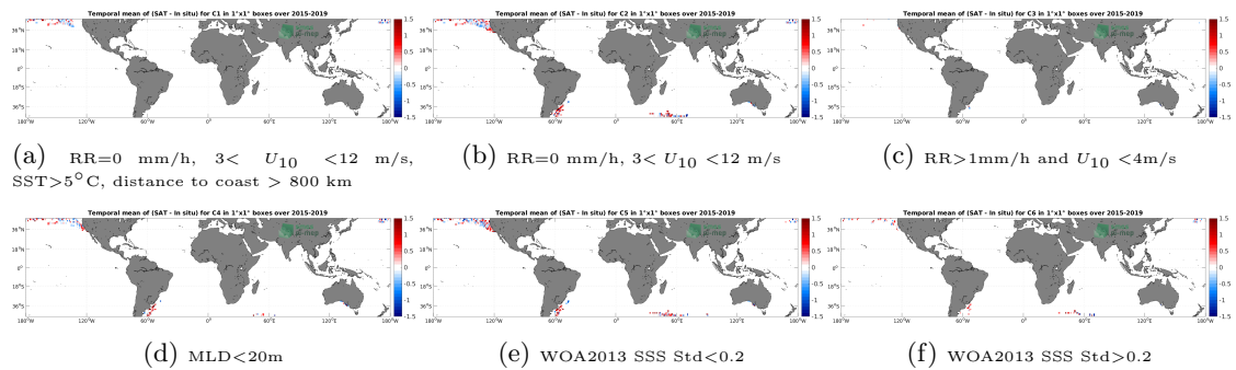
Figure 12: Temporal mean gridded over spatial boxes of size 1^\circ \times 1^\circ of \Delta SSS (SMAP SSS L2 v5.0 (JPL) - Marine mammals) for 6 different subdatasets corresponding to:RR=0 mm/h, 3 < U_{10} < 12 m/s, SST >5^\circ\text{C} , distance to coast > 800 km (a), RR=0 mm/h, 3 < U_{10} < 12 m/s (b), RR >1 mm/h and U_{10} < 4 m/s (c),MLD <20 m (d),WOA2013 SSS Std <0.2 (e),WOA2013 SSS Std >0.2 (f).
