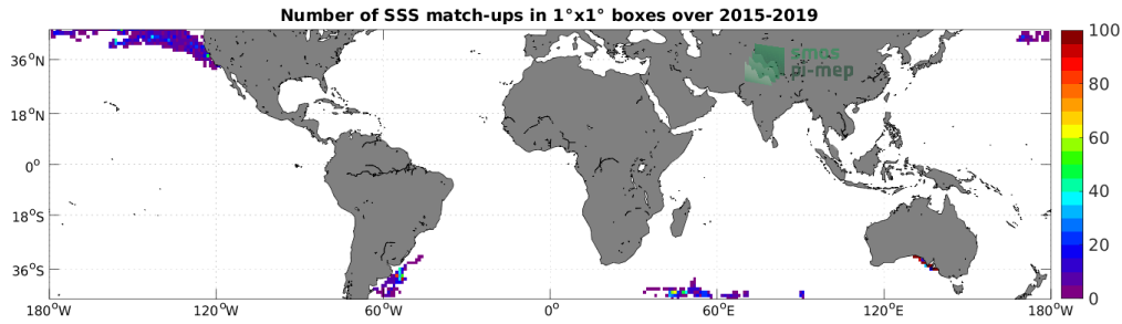
Figure 4: Number of SSS match-ups between Marine mammals SSS and the SMAP SSS L2 v5.0 (JPL) SSS product for the Mid-Low Latitudes 45N-45S Pi-MEP region over 1^\circ \times 1^\circ boxes and for the full satellite product period.
