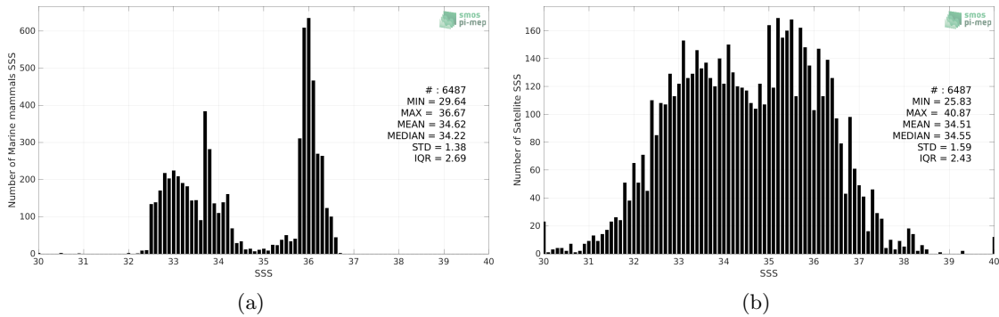
Figure 2: Histograms of SSS from Marine mammals (a) and SMAP SSS L2 v5.0 (JPL) (b) considering all match-up pairs per bins of 0.1 over the Mid-Low Latitudes 45N-45S Pi-MEP region and for the full satellite product period.
