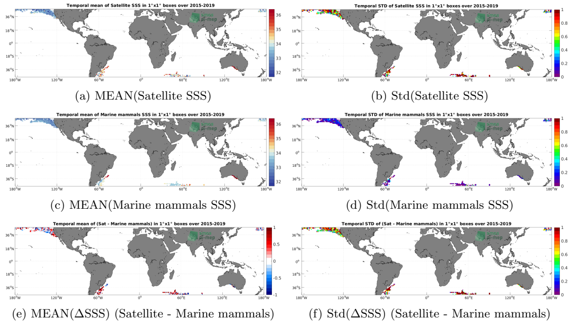
Figure 6: Temporal mean (left) and Std (right) of SSS from SMAP SSS L2 v5.0 (JPL) (top), Marine mammals (middle), and of \Delta SSS (Satellite - Marine mammals). Only match-up pairs are used to generate these maps.
