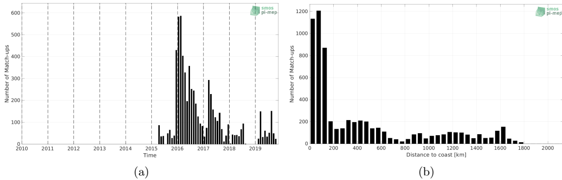
Figure 1: Number of match-ups between Marine mammals and SMAP SSS L2 v5.0 (JPL) SSS as a function of time (a) and as function of the distance to coast (b) over the Mid-Low Latitudes 45N-45S Pi-MEP region and for the full satellite product period.
