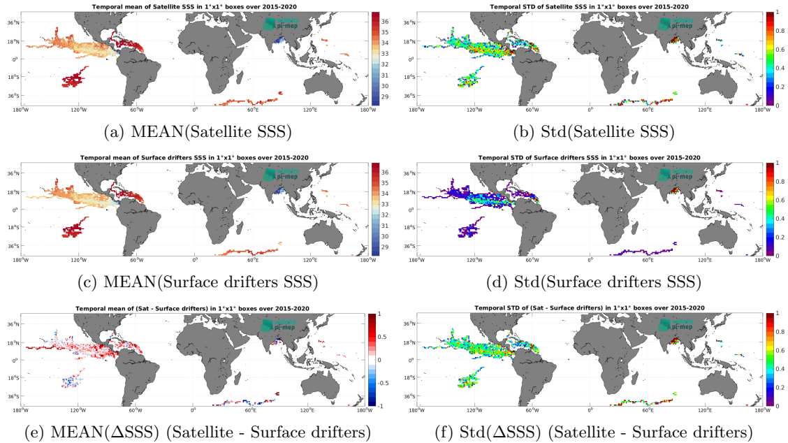
Figure 6: Temporal mean (left) and Std (right) of SSS from SMAP SSS L2 v5.0 (JPL) (top), Surface drifters (middle), and of \Delta\text{SSS} (Satellite - Surface drifters). Only match-up pairs are used to generate these maps.
