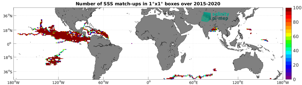
Figure 4: Number of SSS match-ups between Surface drifters SSS and the SMAP SSS L2 v5.0 (JPL) SSS product for the Mid-Low Latitudes 45N-45S Pi-MEP region over 1^\circ \times 1^\circ boxes and for the full satellite product period.
