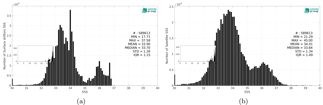
Figure 3: Histograms of SSS from Surface drifters (a) and SMAP SSS L2 v5.0 (JPL) (b) considering all match-up pairs per bins of 0.1 over the Mid-Low Latitudes 45N-45S Pi-MEP region and for the full satellite product period.
