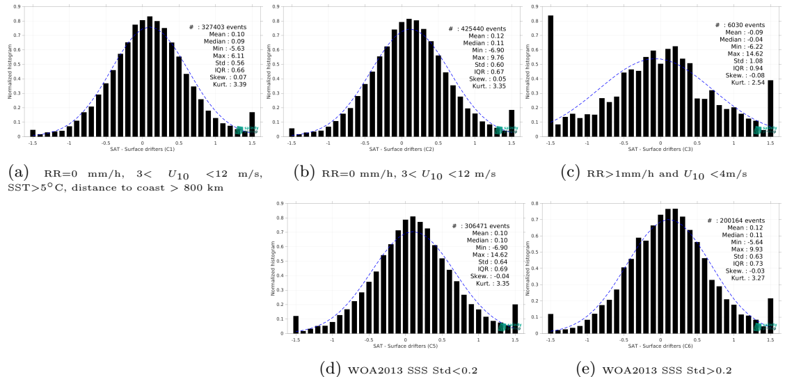
Figure 14: Normalized histogram of \Delta SSS (SMAP SSS L2 v5.0 (JPL) - Surface drifters) for 5 different subdatasets corresponding to: RR=0 mm/h, 3 < U_{10} < 12 m/s, SST >5^\circ\text{C} , distance to coast > 800 km (a), RR=0 mm/h, 3 < U_{10} < 12 m/s (b), RR >1 mm/h and U_{10} < 4 m/s (c), WOA2013 SSS Std <0.2 (d), WOA2013 SSS Std >0.2 (e).
