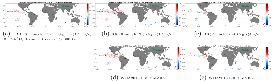
Figure 13: Temporal mean gridded over spatial boxes of size 1^\circ \times 1^\circ of \Delta SSS (SMAP SSS L2 v5.0 (JPL) - Surface drifters) for 5 different subdatasets corresponding to:RR=0 mm/h, 3 < U_{10} < 12 m/s, SST >5^\circ\text{C} , distance to coast > 800 km (a), RR=0 mm/h, 3 < U_{10} < 12 m/s (b), RR >1 mm/h and U_{10} < 4 m/s (c), WOA2013 SSS Std <0.2 (d), WOA2013 SSS Std >0.2 (e).
