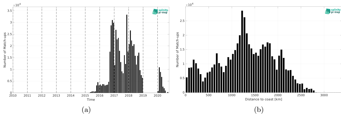
Figure 2: Number of match-ups between Surface drifters and SMAP SSS L2 v5.0 (JPL) SSS as a function of time (a) and as function of the distance to coast (b) over the Mid-Low Latitudes 45N-45S Pi-MEP region and for the full satellite product period.
