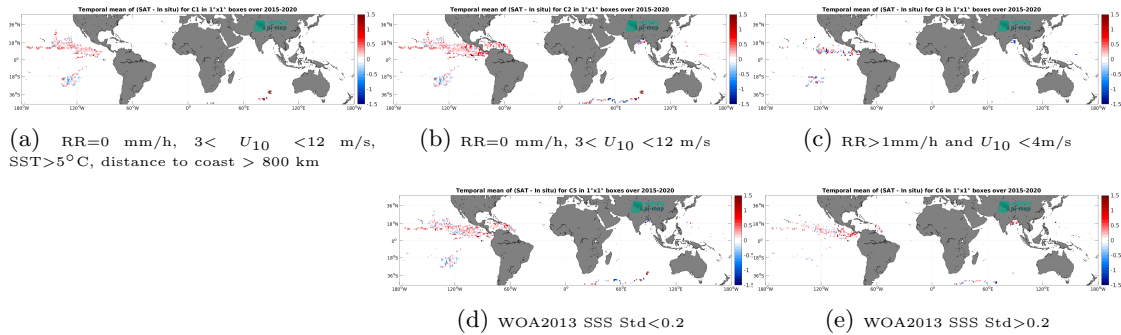
Figure 13: Temporal mean gridded over spatial boxes of size 1°×1° of ΔSSS (SMAP SSS L2 v5.0 (JPL) - Surface drifters) for 5 different subdatasets corresponding to:RR=0 mm/h, 3< U 10 <12 m/s, SST>5°C, distance to coast > 800 km (a), RR=0 mm/h, 3< U 10 <12 m/s (b), RR>1mm/h and U 10 <4m/s (c), WOA2013 SSS Std<0.2 (d), WOA2013 SSS Std>0.2 (e).
