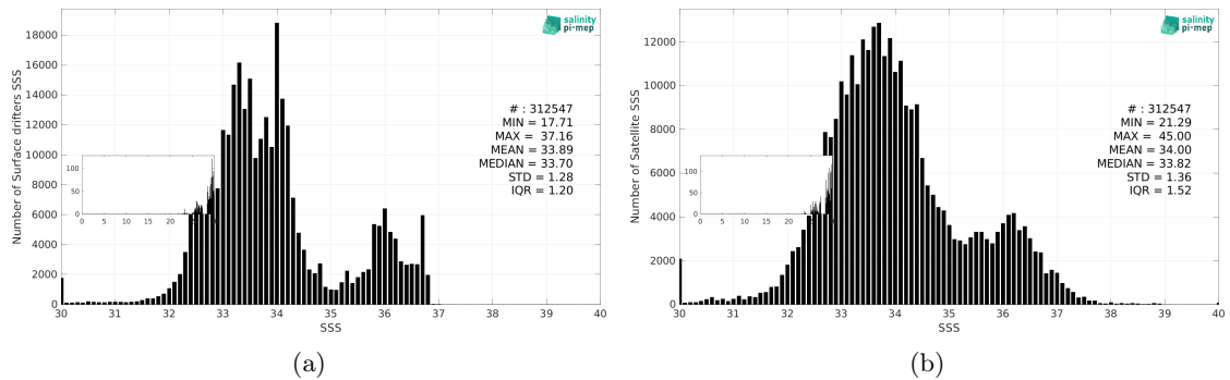
Figure 3: Histograms of SSS from Surface drifters (a) and SMAP SSS L2 v5.0 (JPL) (b) considering all match-up pairs per bins of 0.1 over the Mid-Low Latitudes 45N-45S Pi-MEP region and for the full satellite product period.
