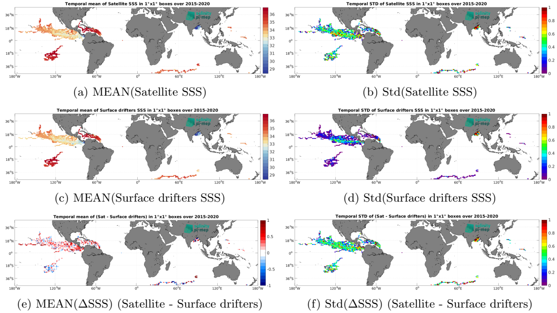
Figure 6: Temporal mean (left) and Std (right) of SSS from SMAP SSS L2 v5.0 (JPL) (top), Surface drifters (middle), and of \Delta\text{SSS} (Satellite - Surface drifters). Only match-up pairs are used to generate these maps.
