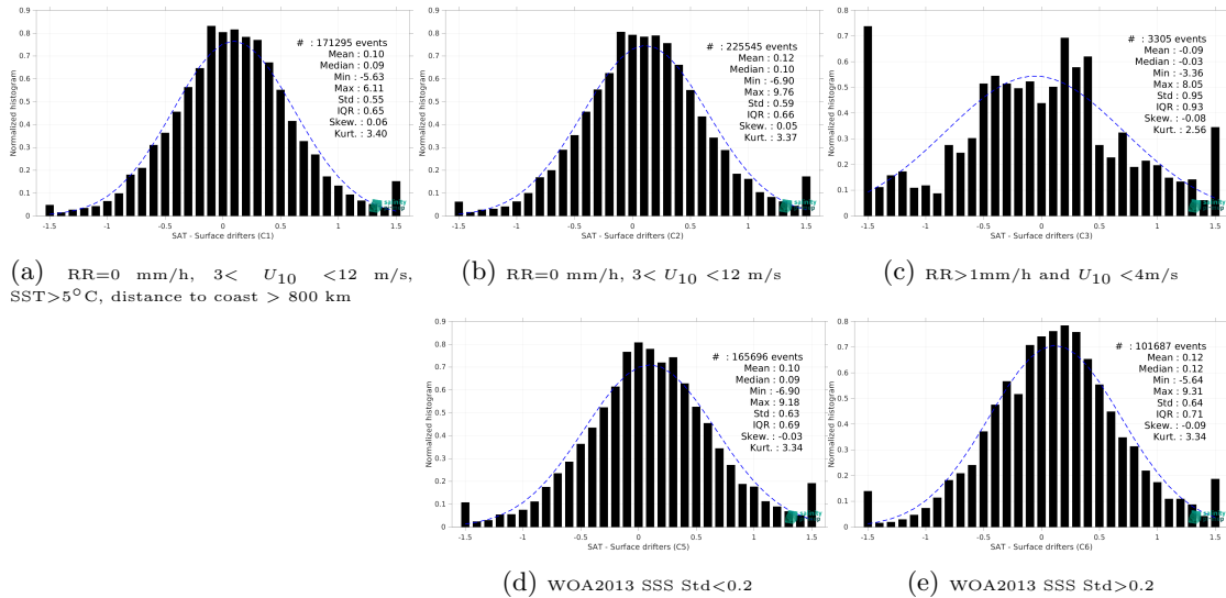
Figure 14: Normalized histogram of ΔSSS (SMAP SSS L2 v5.0 (JPL) - Surface drifters) for 5 different subdatasets corresponding to: RR=0 mm/h, 3< U 10 <12 m/s, SST>5°C, distance to coast > 800 km (a), RR=0 mm/h, 3< U 10 <12 m/s (b), RR>1mm/h and U 10 <4m/s (c), WOA2013 SSS Std<0.2 (d), WOA2013 SSS Std>0.2 (e).
