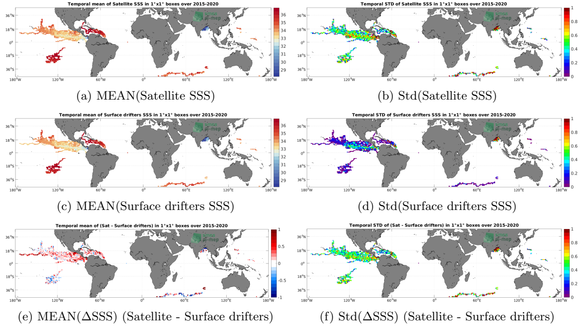
Figure 5: Temporal mean (left) and Std (right) of SSS from SMAP SSS L2 v5.0 (JPL) (top), Surface drifters (middle), and of \Delta\text{SSS} (Satellite - Surface drifters). Only match-up pairs are used to generate these maps.
