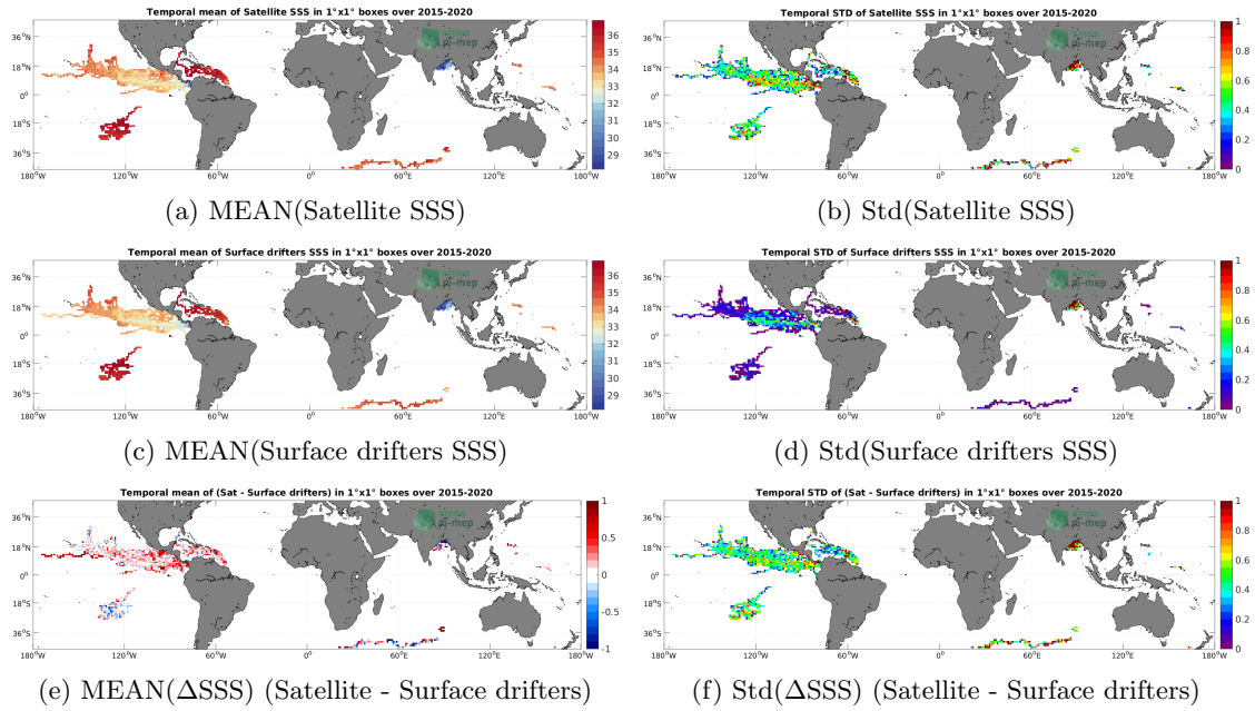
Figure 5: Temporal mean (left) and Std (right) of SSS from SMAP SSS L2 v5.0 (JPL) (top), Surface drifters (middle), and of \Delta SSS (Satellite - Surface drifters). Only match-up pairs are used to generate these maps.
