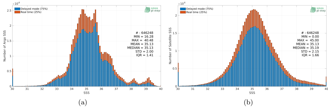
Figure 2: Histograms of SSS from Argo (a) and SMAP SSS L2 v5.0 (JPL) (b) considering all match-up pairs per bins of 0.1 over the Mid-Low Latitudes 45N-45S Pi-MEP region and for the full satellite product period.
