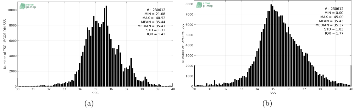
Figure 2: Histograms of SSS from TSG-LEGOS-DM (a) and SMAP-L2-JPL-V4 (b) considering all match-up pairs per bins of 0.1 over the Mid-Low Latitudes 45N-45S Pi-MEP region and for the full satellite product period.
