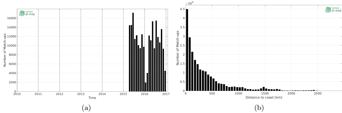
Figure 1: Number of match-ups between TSG-LEGOS-DM and SMAP-L2-JPL-V4 SSS as a function of time (a) and as function of the distance to coast (b) over the Mid-Low Latitudes 45N-45S Pi-MEP region and for the full satellite product period.
