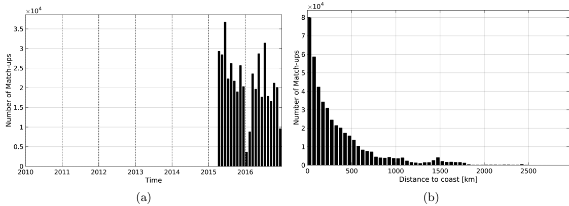
Figure 1: Number of match-ups between TSG-LEGOS-DM and SMAP-L2-JPL-V4 SSS as a function of time (a) and as function of the distance to coast (b) over the Mid-Low Latitudes 45N-45S Pi-MEP region and for the full satellite product period.
