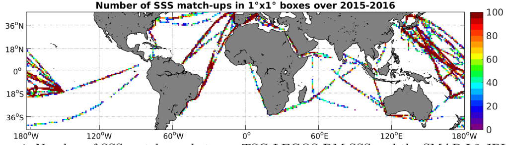
Figure 4: Number of SSS match-ups between TSG-LEGOS-DM SSS and the SMAP-L2-JPL-V4 SSS product for the Mid-Low Latitudes 45N-45S Pi-MEP region over 1^\circ \times 1^\circ boxes and for the full satellite product period.
