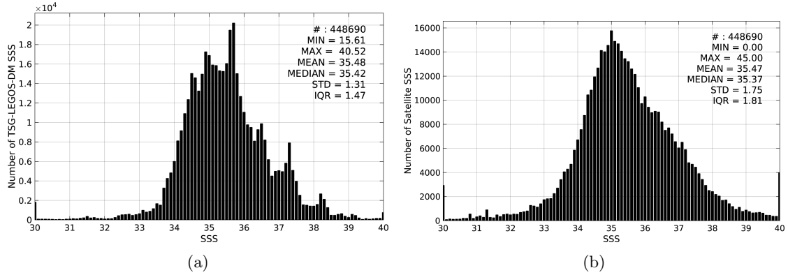
Figure 2: Histograms of SSS from TSG-LEGOS-DM (a) and SMAP-L2-JPL-V4 (b) considering all match-up pairs per bins of 0.1 over the Mid-Low Latitudes 45N-45S Pi-MEP region and for the full satellite product period.
