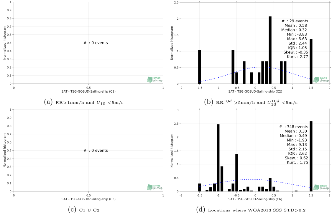
Figure 13: Normalized histogram of \Delta SSS (SMAP-L2-JPL-V4 - TSG-GOSUD-Sailing-ship) for 6 different subdatasets corresponding to: RR > 1\text{mm/h} and U_{10} < 5\text{m/s} (a), RR^{10d} > 5\text{mm/h} and U_{10}^{10d} < 5\text{m/s} (b), C1 \cup C2 (c), Locations where WOA2013 SSS STD > 0.2 (d).
