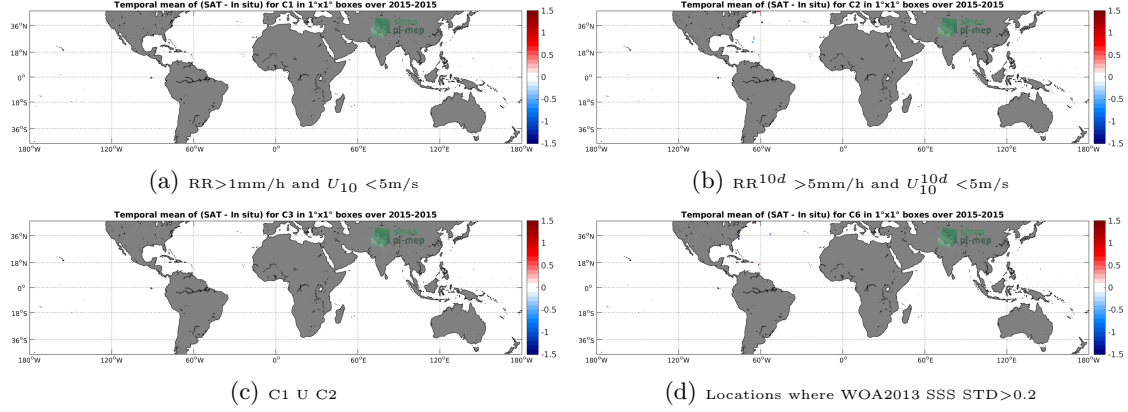
Figure 12: Temporal mean gridded over spatial boxes of size 1^\circ \times 1^\circ of \Delta SSS (SMAP-L2-JPL-V4 - TSG-GOSUD-Sailing-ship) for 4 different subdatasets corresponding to: RR > 1\text{mm/h} and U_{10} < 5\text{m/s} (a), RR^{10d} > 5\text{mm/h} and U_{10}^{10d} < 5\text{m/s} (b), C1 U C2 (c), Locations where WOA2013 SSS STD > 0.2 (d).
