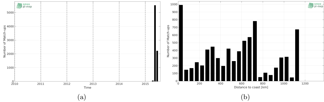
Figure 1: Number of match-ups between TSG-GOSUD-Sailing-ship and SMAP-L2-JPL-V4 SSS as a function of time (a) and as function of the distance to coast (b) over the Mid-Low Latitudes 45N-45S Pi-MEP region and for the full satellite product period.
