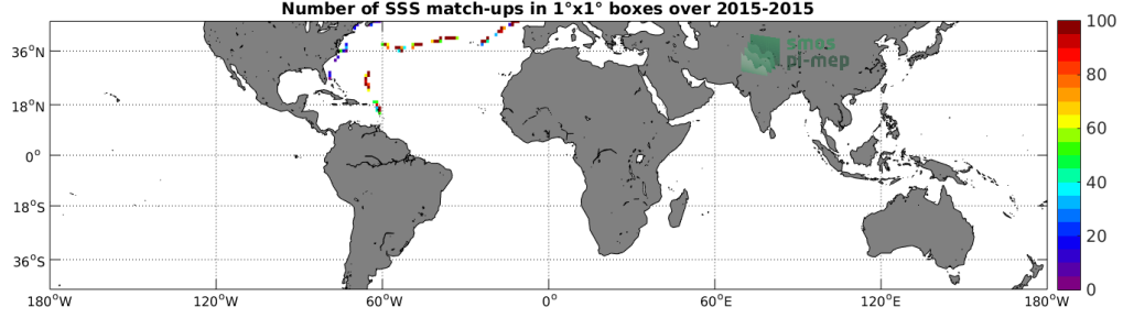
Figure 4: Number of SSS match-ups between TSG-GOSUD-Sailing-ship SSS and the SMAP-L2-JPL-V4 SSS product for the Mid-Low Latitudes 45N-45S Pi-MEP region over 1°x1° boxes and for the full satellite product period.
