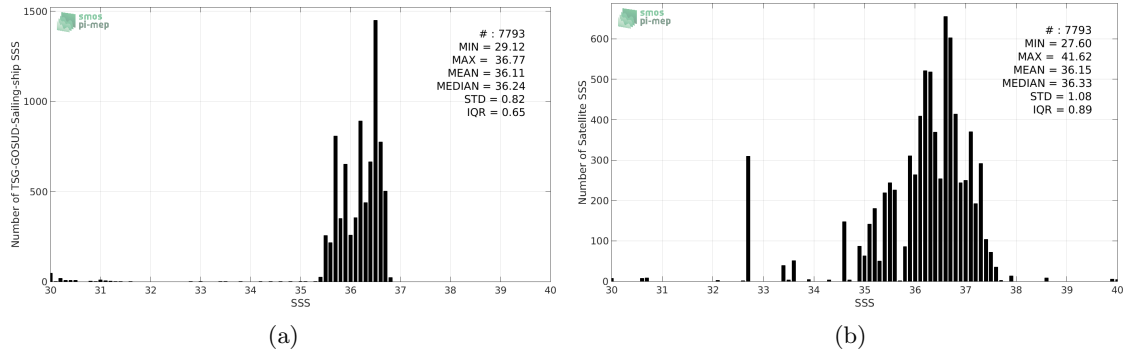
Figure 2: Histograms of SSS from TSG-GOSUD-Sailing-ship (a) and SMAP-L2-JPL-V4 (b) considering all match-up pairs per bins of 0.1 over the Mid-Low Latitudes 45N-45S Pi-MEP region and for the full satellite product period.
