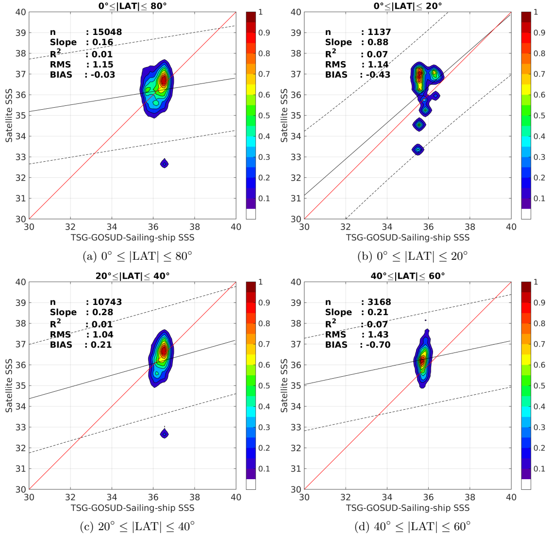
Figure 9: Contour maps of the concentration of SMAP-L2-JPL-V4 SSS (y-axis) versus TSG-GOSUD-Sailing-ship SSS (x-axis) at match-up pairs for different latitude bands. For each plot, the red line shows x=y . The black thin and dashed lines indicate a linear fit through the data cloud and the \pm 95\% confidence levels, respectively. The number match-up pairs n , the slope and R^2 coefficient of the linear fit, the root mean square (RMS) and the mean bias between satellite and in situ data are indicated for each latitude band in each plots.
