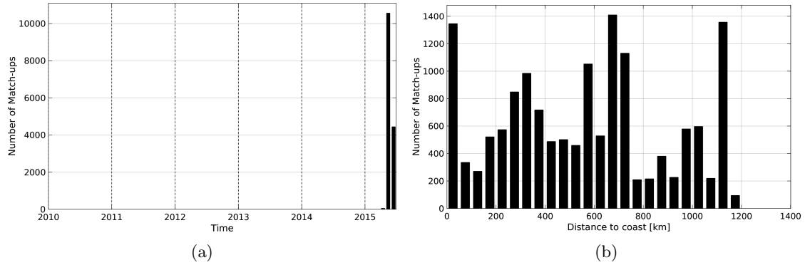
Figure 1: Number of match-ups between TSG-GOSUD-Sailing-ship and SMAP-L2-JPL-V4 SSS as a function of time (a) and as function of the distance to coast (b) over the Mid-Low Latitudes 45N-45S Pi-MEP region and for the full satellite product period.
