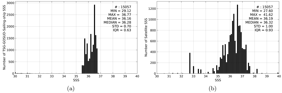
Figure 2: Histograms of SSS from TSG-GOSUD-Sailing-ship (a) and SMAP-L2-JPL-V4 (b) considering all match-up pairs per bins of 0.1 over the Mid-Low Latitudes 45N-45S Pi-MEP region and for the full satellite product period.
