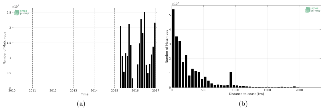
Figure 1: Number of match-ups between TSG-GOSUD-Research-vessel and SMAP-L2-JPL-V4 SSS as a function of time (a) and as function of the distance to coast (b) over the Mid-Low Latitudes 45N-45S Pi-MEP region and for the full satellite product period.
