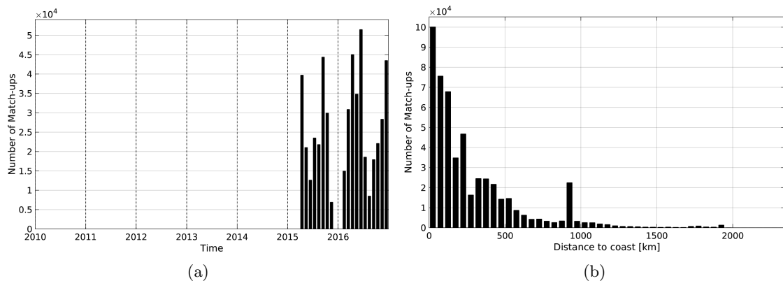
Figure 1: Number of match-ups between TSG-GOSUD-Research-vessel and SMAP-L2-JPL-V4 SSS as a function of time (a) and as function of the distance to coast (b) over the Mid-Low Latitudes 45N-45S Pi-MEP region and for the full satellite product period.
