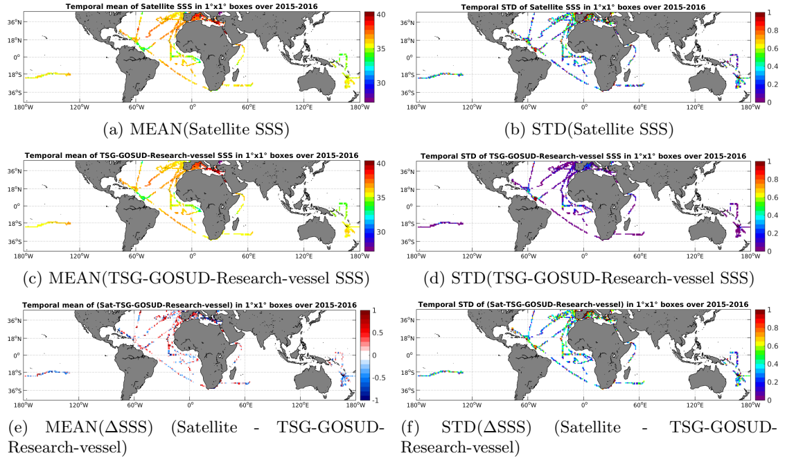
Figure 6: Temporal mean (left) and STD (right) of SSS from SMAP-L2-JPL-V4 (top), TSG-GOSUD-Research-vessel (middle), and of \Delta SSS (Satellite - TSG-GOSUD-Research-vessel). Only match-up pairs are used to generate these maps.
