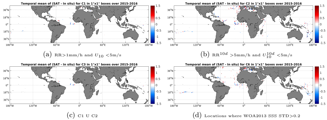
Figure 12: Temporal mean gridded over spatial boxes of size 1^\circ \times 1^\circ of \Delta SSS (SMAP-L2-JPL-V4 - TSG-GOSUD-Research-vessel) for 4 different subdatasets corresponding to: RR > 1\text{mm/h} and U_{10} < 5\text{m/s} (a), RR^{10d} > 5\text{mm/h} and U_{10}^{10d} < 5\text{m/s} (b), C1 U C2 (c), Locations where WOA2013 SSS STD > 0.2 (d).
