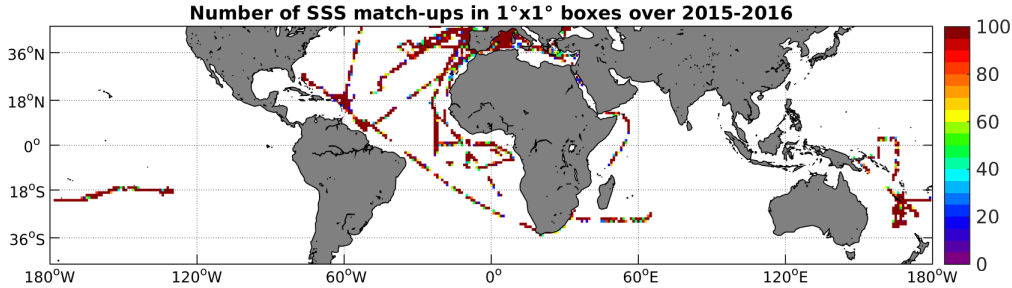
Figure 4: Number of SSS match-ups between TSG-GOSUD-Research-vessel SSS and the SMAP-L2-JPL-V4 SSS product for the Mid-Low Latitudes 45N-45S Pi-MEP region over 1^\circ \times 1^\circ boxes and for the full satellite product period.
