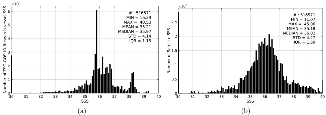
Figure 2: Histograms of SSS from TSG-GOSUD-Research-vessel (a) and SMAP-L2-JPL-V4 (b) considering all match-up pairs per bins of 0.1 over the Mid-Low Latitudes 45N-45S Pi-MEP region and for the full satellite product period.
