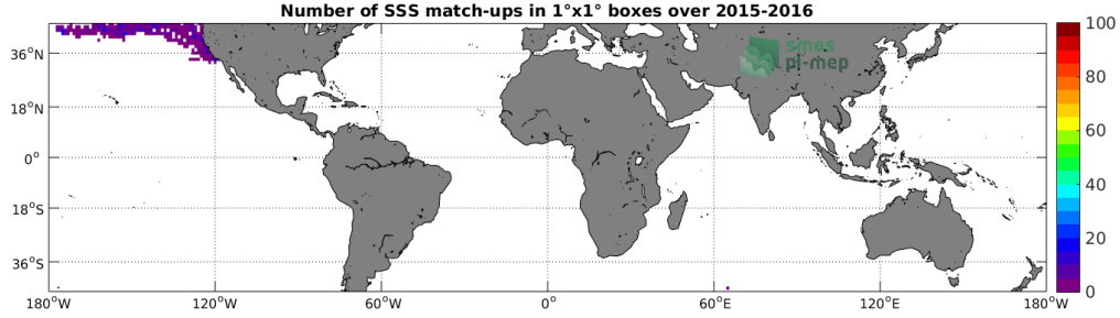
Figure 4: Number of SSS match-ups between Sea mammals SSS and the SMAP-L2-JPL-V4 SSS product for the Mid-Low Latitudes 45N-45S Pi-MEP region over 1°x1° boxes and for the full satellite product period.
