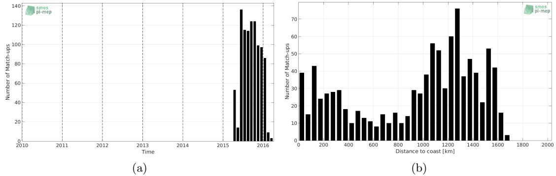
Figure 1: Number of match-ups between Sea mammals and SMAP-L2-JPL-V4 SSS as a function of time (a) and as function of the distance to coast (b) over the Mid-Low Latitudes 45N-45S Pi-MEP region and for the full satellite product period.
