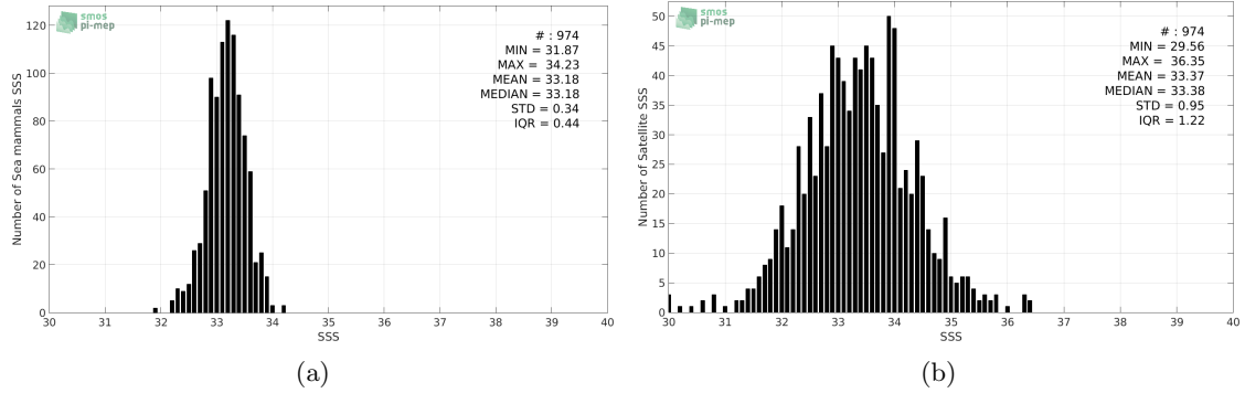
Figure 2: Histograms of SSS from Sea mammals (a) and SMAP-L2-JPL-V4 (b) considering all match-up pairs per bins of 0.1 over the Mid-Low Latitudes 45N-45S Pi-MEP region and for the full satellite product period.
