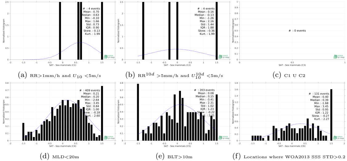
Figure 13: Normalized histogram of \Delta\text{SSS} (SMAP-L2-JPL-V4 - Sea mammals) for 6 different subdatasets corresponding to: \text{RR} > 1\text{mm/h} and U_{10} < 5\text{m/s} (a), \text{RR}^{10d} > 5\text{mm/h} and U_{10}^{10d} < 5\text{m/s} (b), C1 U C2 (c), \text{MLD} < 20\text{m} (d), \text{BLT} > 10\text{m} (e), Locations where WOA2013 SSS STD > 0.2 (f).
