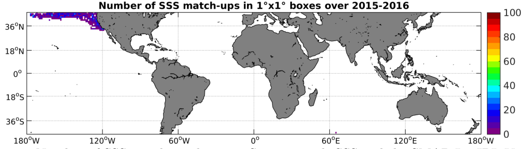
Figure 4: Number of SSS match-ups between Sea mammals SSS and the SMAP-L2-JPL-V4 SSS product for the Mid-Low Latitudes 45N-45S Pi-MEP region over 1^\circ \times 1^\circ boxes and for the full satellite product period.
