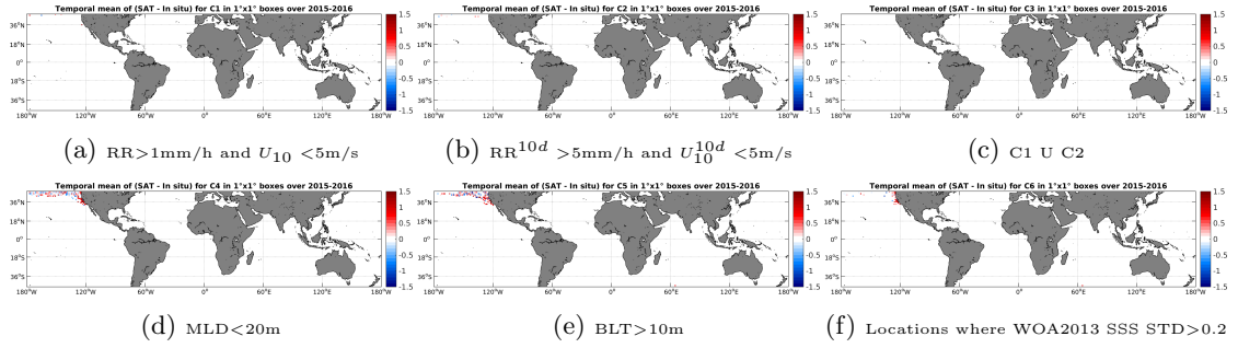
Figure 12: Temporal mean gridded over spatial boxes of size 1^\circ \times 1^\circ of \Delta SSS (SMAP-L2-JPL-V4 - Sea mammals) for 6 different subdatasets corresponding to: RR > 1\text{mm/h} and U_{10} < 5\text{m/s} (a), RR^{10d} > 5\text{mm/h} and U_{10}^{10d} < 5\text{m/s} (b), C1 U C2 (c), MLD < 20\text{m} (d), BLT > 10\text{m} (e), Locations where WOA2013 SSS STD > 0.2 (f).
