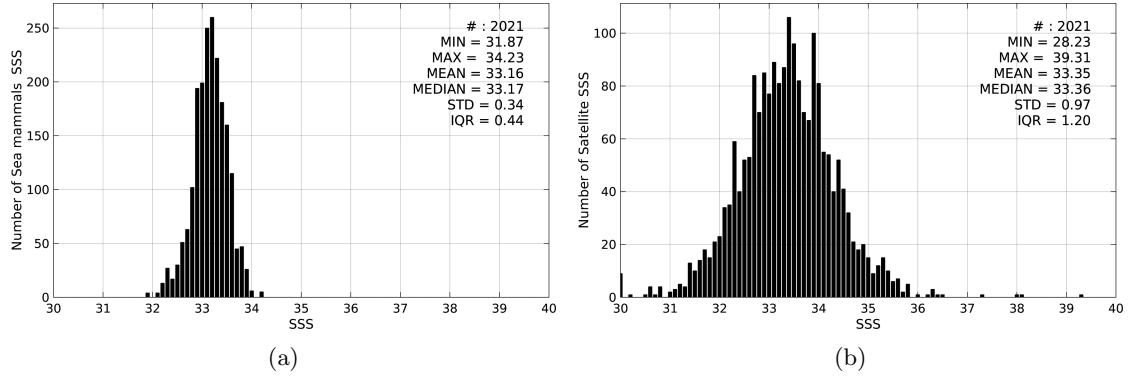
Figure 2: Histograms of SSS from Sea mammals (a) and SMAP-L2-JPL-V4 (b) considering all match-up pairs per bins of 0.1 over the Mid-Low Latitudes 45N-45S Pi-MEP region and for the full satellite product period.
