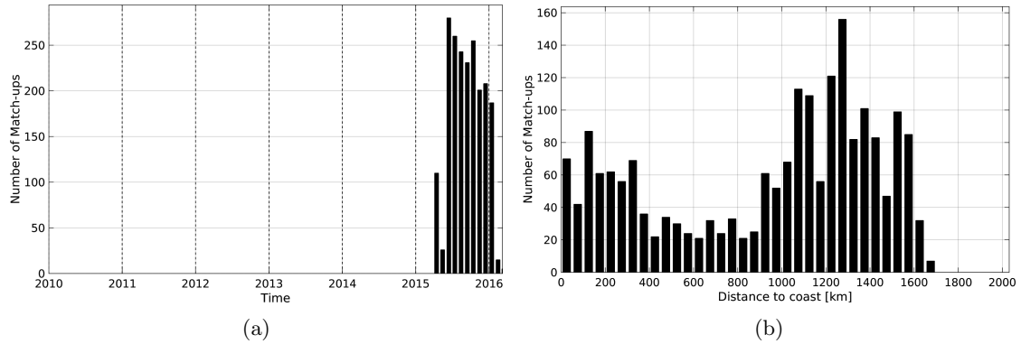
Figure 1: Number of match-ups between Sea mammals and SMAP-L2-JPL-V4 SSS as a function of time (a) and as function of the distance to coast (b) over the Mid-Low Latitudes 45N-45S Pi-MEP region and for the full satellite product period.
