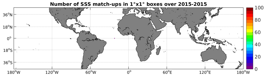
Figure 3: Number of SSS match-ups between Surface drifters SSS and the SMAP-L2-JPL-V4 SSS product for the Mid-Low Latitudes 45N-45S Pi-MEP region over 1°x1° boxes and for the full satellite product period.
