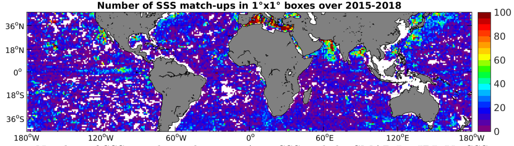
Figure 4: Number of SSS match-ups between Argo SSS and the SMAP-L2-JPL-V4 SSS product for the Mid-Low Latitudes 45N-45S Pi-MEP region over 1°x1° boxes and for the full satellite product period.
