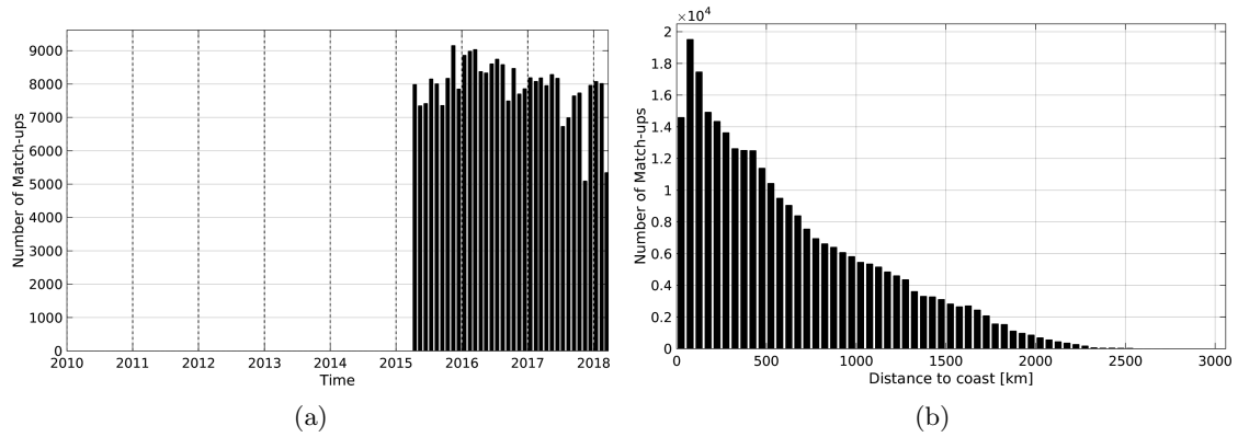
Figure 1: Number of match-ups between Argo and SMAP-L2-JPL-V4 SSS as a function of time (a) and as function of the distance to coast (b) over the Mid-Low Latitudes 45N-45S Pi-MEP region and for the full satellite product period.
