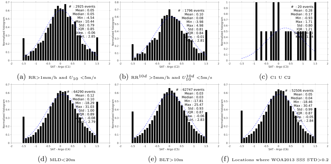
Figure 13: Normalized histogram of \Delta\text{SSS} (SMAP-L2-JPL-V4 - Argo) for 6 different subdatasets corresponding to: RR > 1\text{mm/h} and U_{10} < 5\text{m/s} (a), RR^{10d} > 5\text{mm/h} and U_{10}^{10d} < 5\text{m/s} (b), C1 U C2 (c), MLD < 20\text{m} (d), BLT > 10\text{m} (e), Locations where WOA2013 SSS STD > 0.2 (f).
