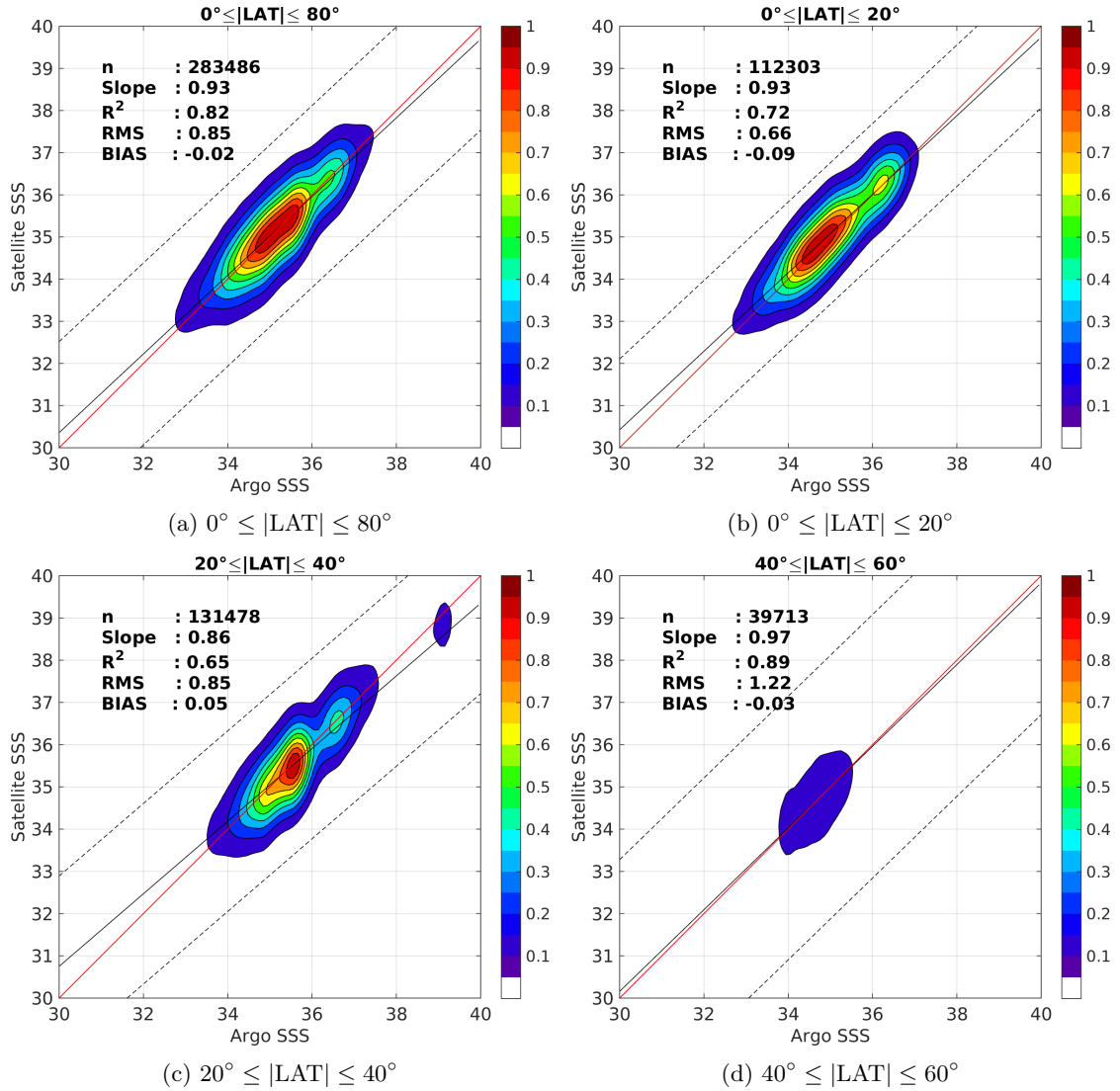
Figure 9: Contour maps of the concentration of SMAP-L2-JPL-V4 SSS (y-axis) versus Argo SSS (x-axis) at match-up pairs for different latitude bands. For each plot, the red line shows x=y . The black thin and dashed lines indicate a linear fit through the data cloud and the \pm 95\% confidence levels, respectively. The number match-up pairs n , the slope and R^2 coefficient of the linear fit, the root mean square (RMS) and the mean bias between satellite and in situ data are indicated for each latitude band in each plots.
