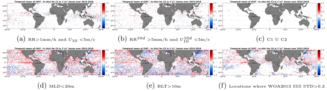
Figure 12: Temporal mean gridded over spatial boxes of size 1^\circ \times 1^\circ of \Delta\text{SSS} (SMAP-L2-JPL-V4 - Argo) for 6 different subdatasets corresponding to: RR > 1\text{mm/h} and U_{10} < 5\text{m/s} (a), RR^{10d} > 5\text{mm/h} and U_{10}^{10d} < 5\text{m/s} (b), C1 U C2 (c), MLD < 20\text{m} (d), BLT > 10\text{m} (e), Locations where WOA2013 SSS STD > 0.2 (f).
