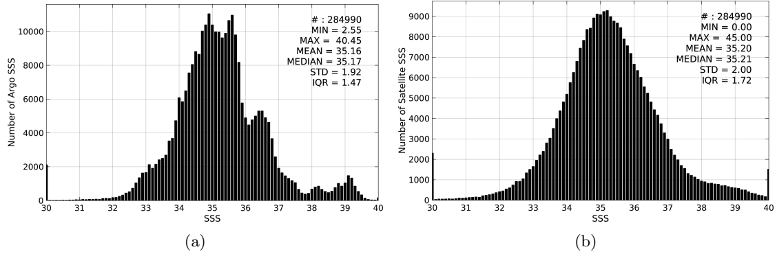
Figure 2: Histograms of SSS from Argo (a) and SMAP-L2-JPL-V4 (b) considering all match-up pairs per bins of 0.1 over the Mid-Low Latitudes 45N-45S Pi-MEP region and for the full satellite product period.
