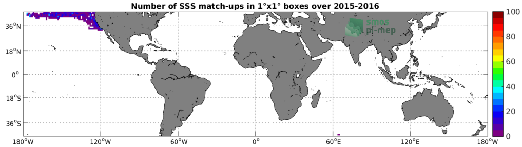
Figure 4: Number of SSS match-ups between Sea mammals SSS and the SMAP-L2-JPL-V4.3 SSS product for the Mid-Low Latitudes 45N-45S Pi-MEP region over 1^\circ \times 1^\circ boxes and for the full satellite product period.
