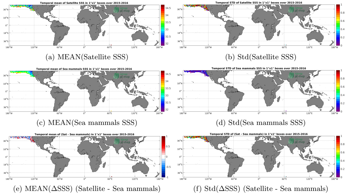
Figure 6: Temporal mean (left) and Std (right) of SSS from SMAP-L2-JPL-V4.3 (top), Sea mammals (middle), and of \Delta SSS (Satellite - Sea mammals). Only match-up pairs are used to generate these maps.
