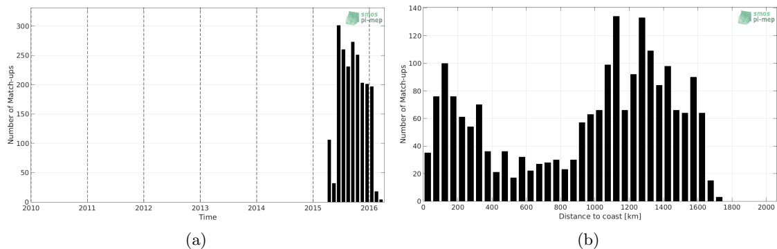
Figure 1: Number of match-ups between Sea mammals and SMAP-L2-JPL-V4.3 SSS as a function of time (a) and as function of the distance to coast (b) over the Mid-Low Latitudes 45N-45S Pi-MEP region and for the full satellite product period.
