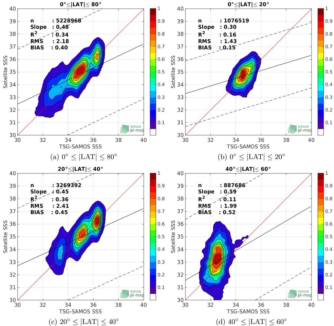
Figure 9: Contour maps of the concentration of SMAP-L2-JPL-V4.2 SSS (y-axis) versus TSG-SAMOS SSS (x-axis) at match-up pairs for different latitude bands. For each plot, the red line shows x=y . The black thin and dashed lines indicate a linear fit through the data cloud and the \pm 95\% confidence levels, respectively. The number match-up pairs n , the slope and R^2 coefficient of the linear fit, the root mean square (RMS) and the mean bias between satellite and in situ data are indicated for each latitude band in each plots.
