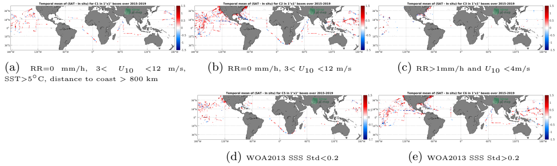
Figure 12: Temporal mean gridded over spatial boxes of size 1^\circ \times 1^\circ of \Delta SSS (SMAP-L2-JPL-V4.2 - TSG-SAMOS) for 5 different subdatasets corresponding to:RR=0 mm/h, 3 < U_{10} < 12 m/s, SST >5^\circ\text{C} , distance to coast > 800 km (a), RR=0 mm/h, 3 < U_{10} < 12 m/s (b), RR >1 mm/h and U_{10} < 4 m/s (c), WOA2013 SSS Std <0.2 (d), WOA2013 SSS Std >0.2 (e).
