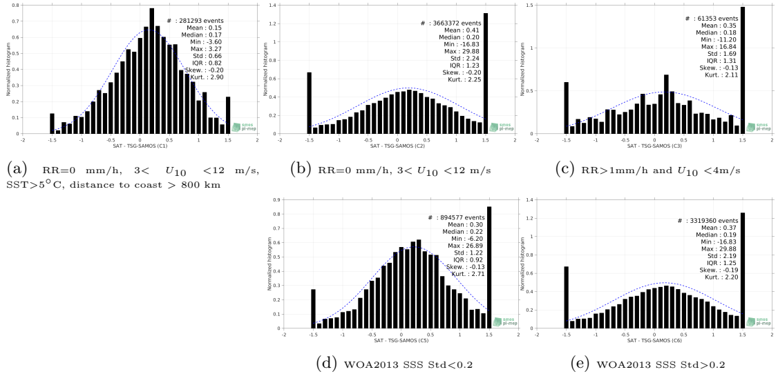
Figure 13: Normalized histogram of \Delta SSS (SMAP-L2-JPL-V4.2 - TSG-SAMOS) for 5 different subdatasets corresponding to: RR=0 mm/h, 3 < U_{10} < 12 m/s, SST >5^\circ\text{C} , distance to coast > 800 km (a), RR=0 mm/h, 3 < U_{10} < 12 m/s (b), RR >1 mm/h and U_{10} < 4 m/s (c), WOA2013 SSS Std <0.2 (d), WOA2013 SSS Std >0.2 (e).
