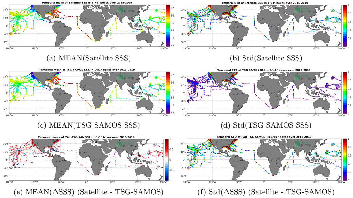
Figure 6: Temporal mean (left) and Std (right) of SSS from SMAP-L2-JPL-V4.2 (top), TSG-SAMOS (middle), and of \Delta SSS (Satellite - TSG-SAMOS). Only match-up pairs are used to generate these maps.
