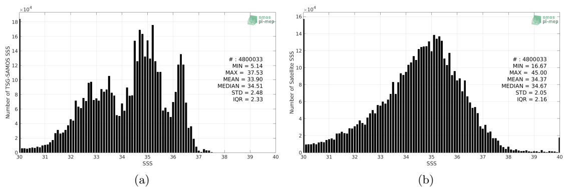
Figure 2: Histograms of SSS from TSG-SAMOS (a) and SMAP-L2-JPL-V4.2 (b) considering all match-up pairs per bins of 0.1 over the Mid-Low Latitudes 45N-45S Pi-MEP region and for the full satellite product period.
