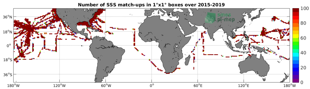
Figure 4: Number of SSS match-ups between TSG-SAMOS SSS and the SMAP-L2-JPL-V4.2 SSS product for the Mid-Low Latitudes 45N-45S Pi-MEP region over 1^\circ \times 1^\circ boxes and for the full satellite product period.
