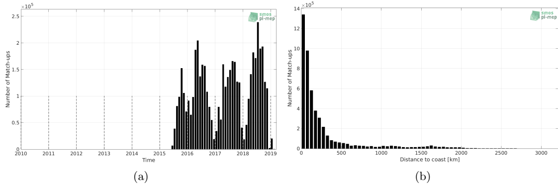
Figure 1: Number of match-ups between TSG-SAMOS and SMAP-L2-JPL-V4.2 SSS as a function of time (a) and as function of the distance to coast (b) over the Mid-Low Latitudes 45N-45S Pi-MEP region and for the full satellite product period.
