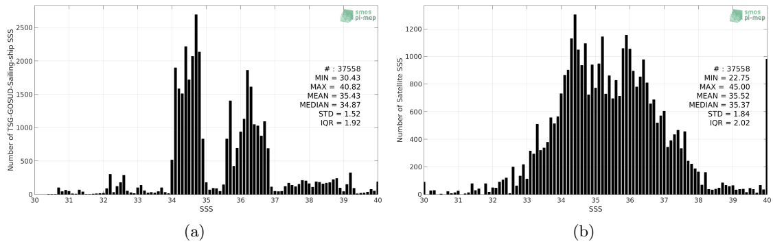
Figure 2: Histograms of SSS from TSG-GOSUD-Sailing-ship (a) and SMAP-L2-JPL-V4.2 (b) considering all match-up pairs per bins of 0.1 over the Mid-Low Latitudes 45N-45S Pi-MEP region and for the full satellite product period.
