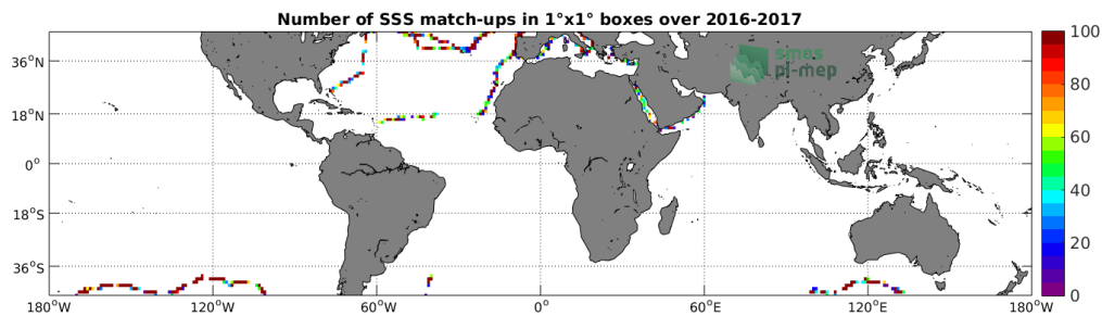
Figure 4: Number of SSS match-ups between TSG-GOSUD-Sailing-ship SSS and the SMAP-L2-JPL-V4.2 SSS product for the Mid-Low Latitudes 45N-45S Pi-MEP region over 1^\circ \times 1^\circ boxes and for the full satellite product period.
