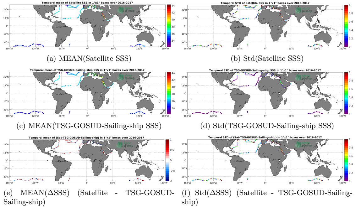
Figure 6: Temporal mean (left) and Std (right) of SSS from SMAP-L2-JPL-V4.2 (top), TSG-GOSUD-Sailing-ship (middle), and of \Delta SSS (Satellite - TSG-GOSUD-Sailing-ship). Only match-up pairs are used to generate these maps.
