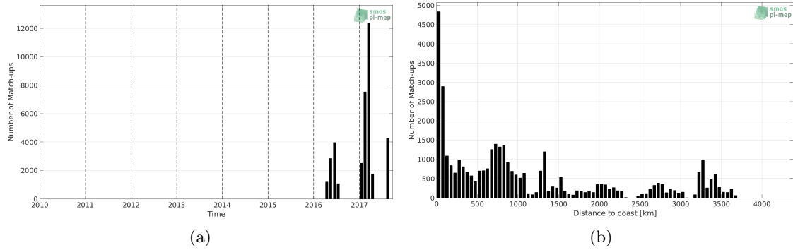
Figure 1: Number of match-ups between TSG-GOSUD-Sailing-ship and SMAP-L2-JPL-V4.2 SSS as a function of time (a) and as function of the distance to coast (b) over the Mid-Low Latitudes 45N-45S Pi-MEP region and for the full satellite product period.
