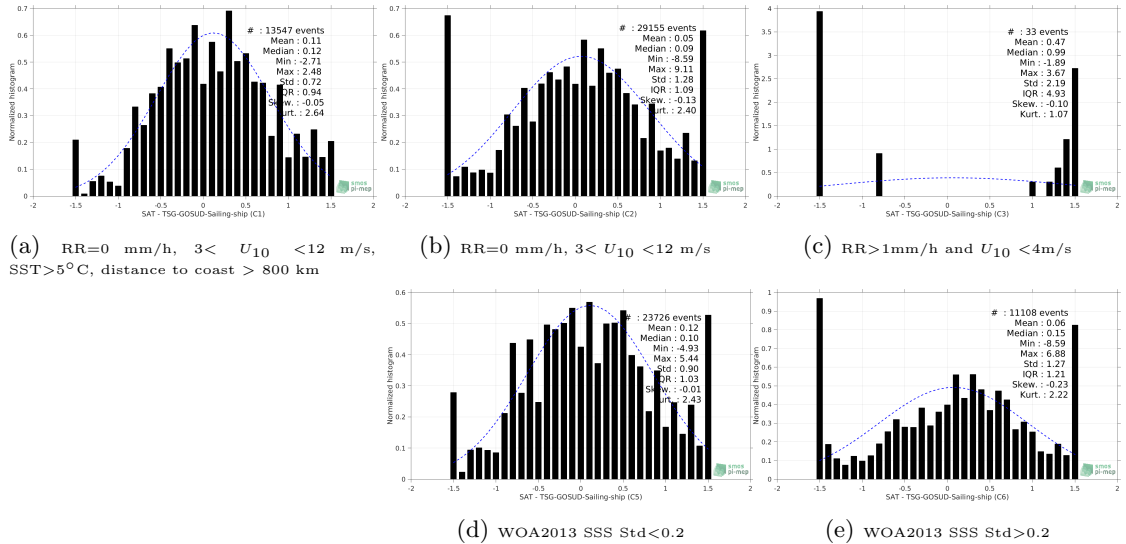
Figure 13: Normalized histogram of \Delta SSS (SMAP-L2-JPL-V4.2 - TSG-GOSUD-Sailing-ship) for 5 different subdatasets corresponding to: RR=0 mm/h, 3 < U_{10} < 12 m/s, SST >5^\circ C, distance to coast > 800 km (a), RR=0 mm/h, 3 < U_{10} < 12 m/s (b), RR >1 mm/h and U_{10} < 4 m/s (c), WOA2013 SSS Std <0.2 (d), WOA2013 SSS Std >0.2 (e).
