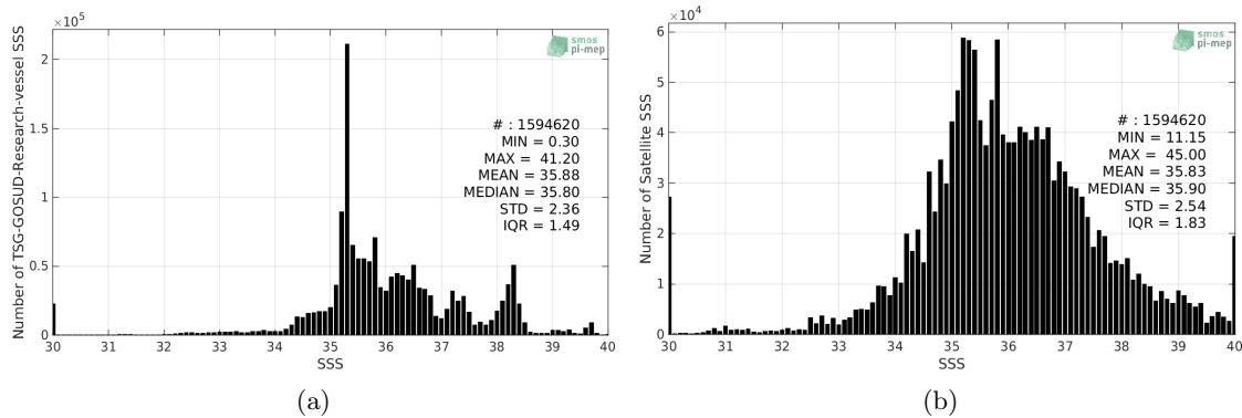
Figure 2: Histograms of SSS from TSG-GOSUD-Research-vessel (a) and SMAP-L2-JPL-V4.2 (b) considering all match-up pairs per bins of 0.1 over the Mid-Low Latitudes 45N-45S Pi-MEP region and for the full satellite product period.
