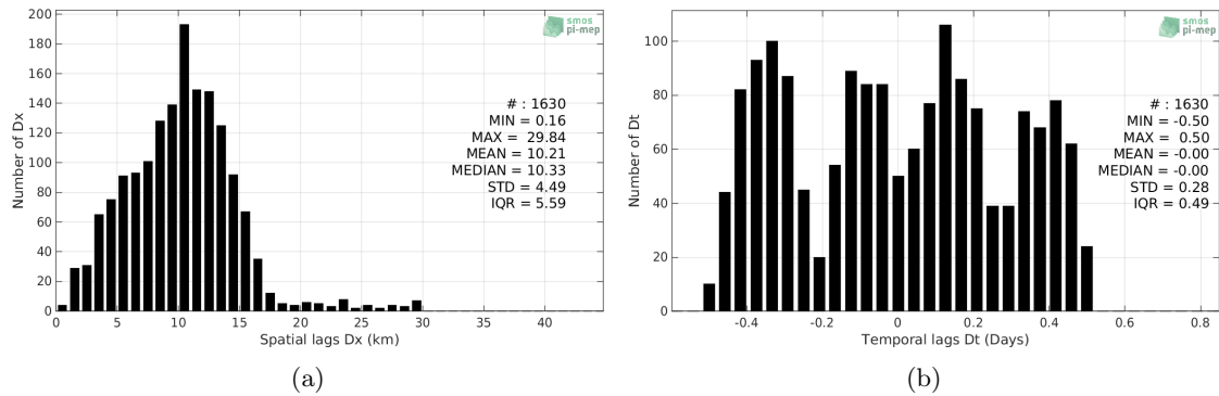
Figure 5: Histograms of the spatial (a) and temporal (b) lags between the time of the Sea mammals measurements and the date of the corresponding SMAP-L2-JPL-V4.2 SSS product.
