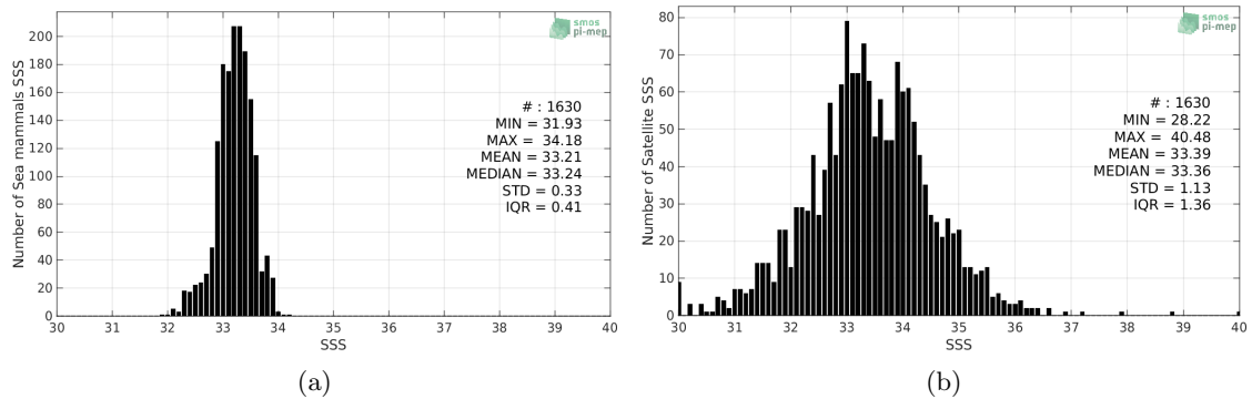
Figure 2: Histograms of SSS from Sea mammals (a) and SMAP-L2-JPL-V4.2 (b) considering all match-up pairs per bins of 0.1 over the Mid-Low Latitudes 45N-45S Pi-MEP region and for the full satellite product period.
