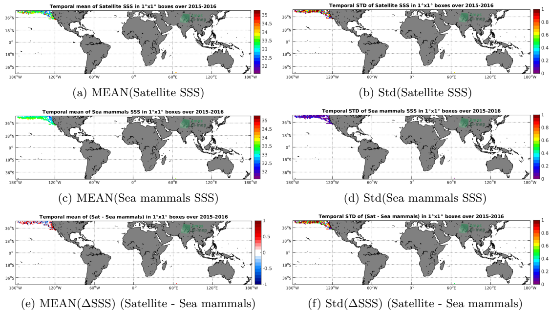
Figure 6: Temporal mean (left) and Std (right) of SSS from SMAP-L2-JPL-V4.2 (top), Sea mammals (middle), and of \Delta SSS (Satellite - Sea mammals). Only match-up pairs are used to generate these maps.
