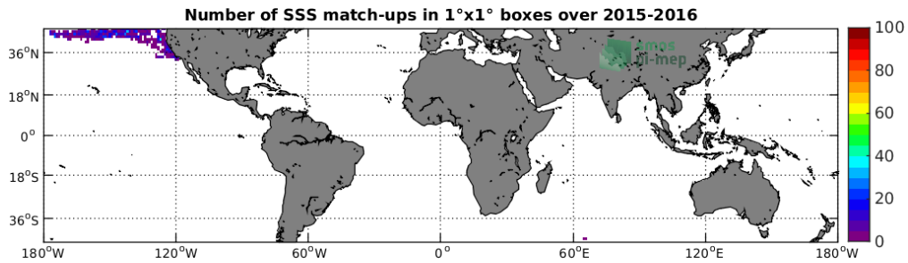
Figure 4: Number of SSS match-ups between Sea mammals SSS and the SMAP-L2-JPL-V4.2 SSS product for the Mid-Low Latitudes 45N-45S Pi-MEP region over 1^\circ \times 1^\circ boxes and for the full satellite product period.
