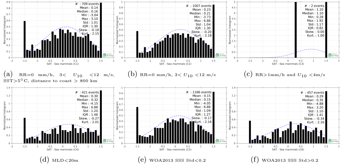
Figure 13: Normalized histogram of \Delta SSS (SMAP-L2-JPL-V4.2 - Sea mammals) for 6 different subdatasets corresponding to: RR=0 mm/h, 3 < U_{10} < 12 m/s, SST > 5°C, distance to coast > 800 km (a), RR=0 mm/h, 3 < U_{10} < 12 m/s (b), RR > 1mm/h and U_{10} < 4 m/s (c), MLD < 20m (d), WOA2013 SSS Std < 0.2 (e), WOA2013 SSS Std > 0.2 (f).
