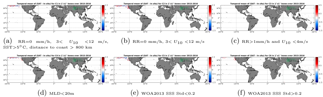
Figure 12: Temporal mean gridded over spatial boxes of size 1^\circ \times 1^\circ of \Delta SSS (SMAP-L2-JPL-V4.2 - Sea mammals) for 6 different subdatasets corresponding to:RR=0 mm/h, 3 < U_{10} < 12 m/s, SST >5^\circ C, distance to coast > 800 km (a), RR=0 mm/h, 3 < U_{10} < 12 m/s (b), RR >1 mm/h and U_{10} < 4 m/s (c),MLD <20 m (d),WOA2013 SSS Std <0.2 (e),WOA2013 SSS Std >0.2 (f).
