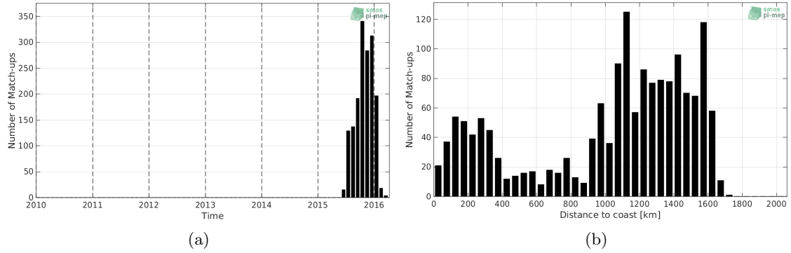
Figure 1: Number of match-ups between Sea mammals and SMAP-L2-JPL-V4.2 SSS as a function of time (a) and as function of the distance to coast (b) over the Mid-Low Latitudes 45N-45S Pi-MEP region and for the full satellite product period.
