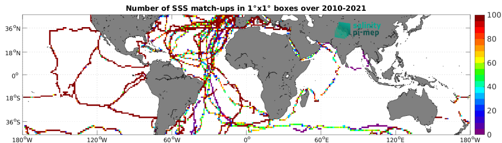
Figure 5: Number of SSS match-ups between TSG (GOSUD-Sailing-ship) SSS and the ISAS v7 - Monthly (Ifremer-LOPS-CMEMS) SSS product for the Mid-Low Latitudes 45N-45S Pi-MEP region over 1^\circ \times 1^\circ boxes and for the full satellite product period.
