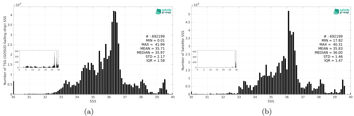
Figure 3: Histograms of SSS from TSG (GOSUD-Sailing-ship) (a) and ISAS v7 - Monthly (Ifremer-LOPS-CMEMS) (b) considering all match-up pairs per bins of 0.1 over the Mid-Low Latitudes 45N-45S Pi-MEP region and for the full satellite product period.
