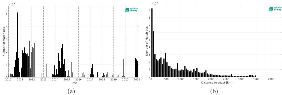
Figure 2: Number of match-ups between TSG (GOSUD-Sailing-ship) and ISAS v7 - Monthly (Ifremer-LOPS-CMEMS) SSS as a function of time (a) and as function of the distance to coast (b) over the Mid-Low Latitudes 45N-45S Pi-MEP region and for the full satellite product period.
