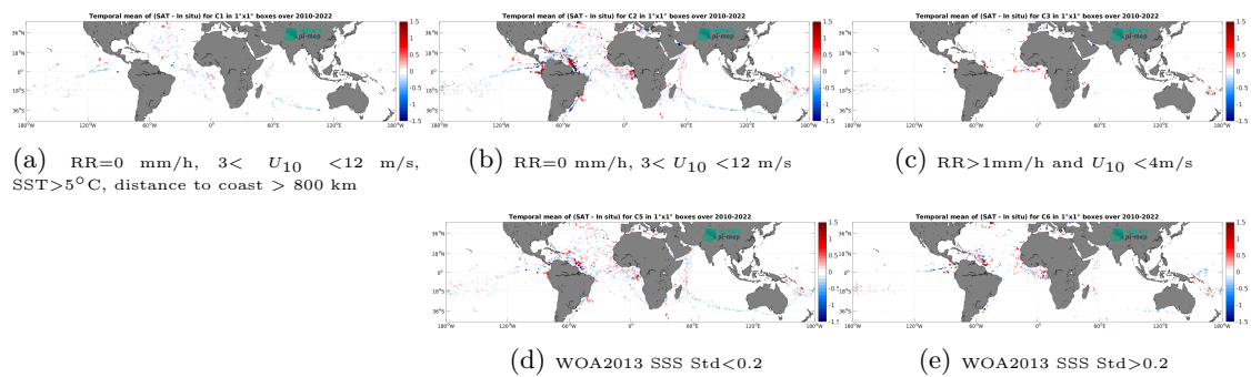
Figure 14: Temporal mean gridded over spatial boxes of size 1^\circ \times 1^\circ of \Delta\text{SSS} (ISAS v7 - Monthly (Ifremer-LOPS-CMEMS) - TSG (GOSUD-Research-vessel)) for 5 different subdatasets corresponding to:RR=0 mm/h, 3 < U_{10} < 12 m/s, SST>5°C, distance to coast > 800 km (a), RR=0 mm/h, 3 < U_{10} < 12 m/s (b), RR>1mm/h and U_{10} < 4 m/s (c), WOA2013 SSS Std<0.2 (d), WOA2013 SSS Std>0.2 (e).
