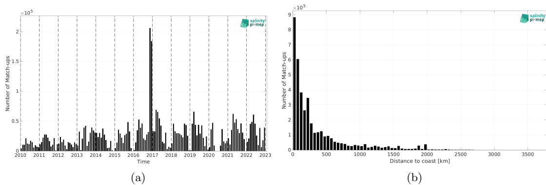
Figure 2: Number of match-ups between TSG (GOSUD-Research-vessel) and ISAS v7 - Monthly (Ifremer-LOPS-CMEMS) SSS as a function of time (a) and as function of the distance to coast (b) over the Mid-Low Latitudes 45N-45S Pi-MEP region and for the full satellite product period.
