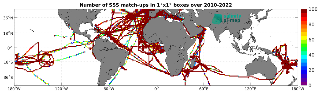
Figure 5: Number of SSS match-ups between TSG (GOSUD-Research-vessel) SSS and the ISAS v7 - Monthly (Ifremer-LOPS-CMEMS) SSS product for the Mid-Low Latitudes 45N-45S Pi-MEP region over 1^\circ \times 1^\circ boxes and for the full satellite product period.
