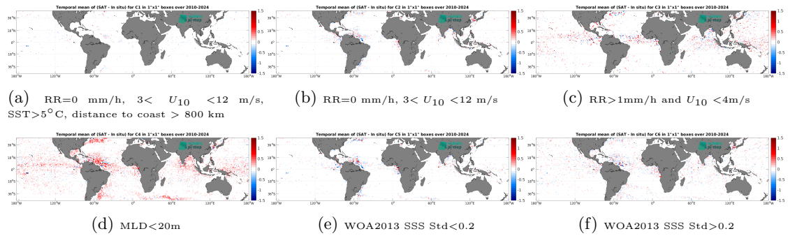
Figure 14: Temporal mean gridded over spatial boxes of size 1^\circ \times 1^\circ of \Delta SSS (ISAS - Argo) for 6 different subdatasets corresponding to:RR=0 mm/h, 3 < U_{10} < 12 m/s, SST >5^\circ\text{C} , distance to coast > 800 km (a), RR=0 mm/h, 3 < U_{10} < 12 m/s (b), RR >1 mm/h and U_{10} < 4 m/s (c),MLD <20 m (d),WOA2013 SSS Std <0.2 (e),WOA2013 SSS Std >0.2 (f).
