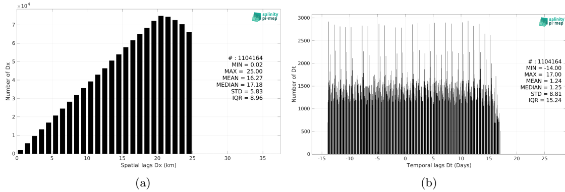
Figure 6: Histograms of the spatial (a) and temporal (b) lags between the location/time of the Argo measurement and the date of the corresponding ISAS SSS pixel.
