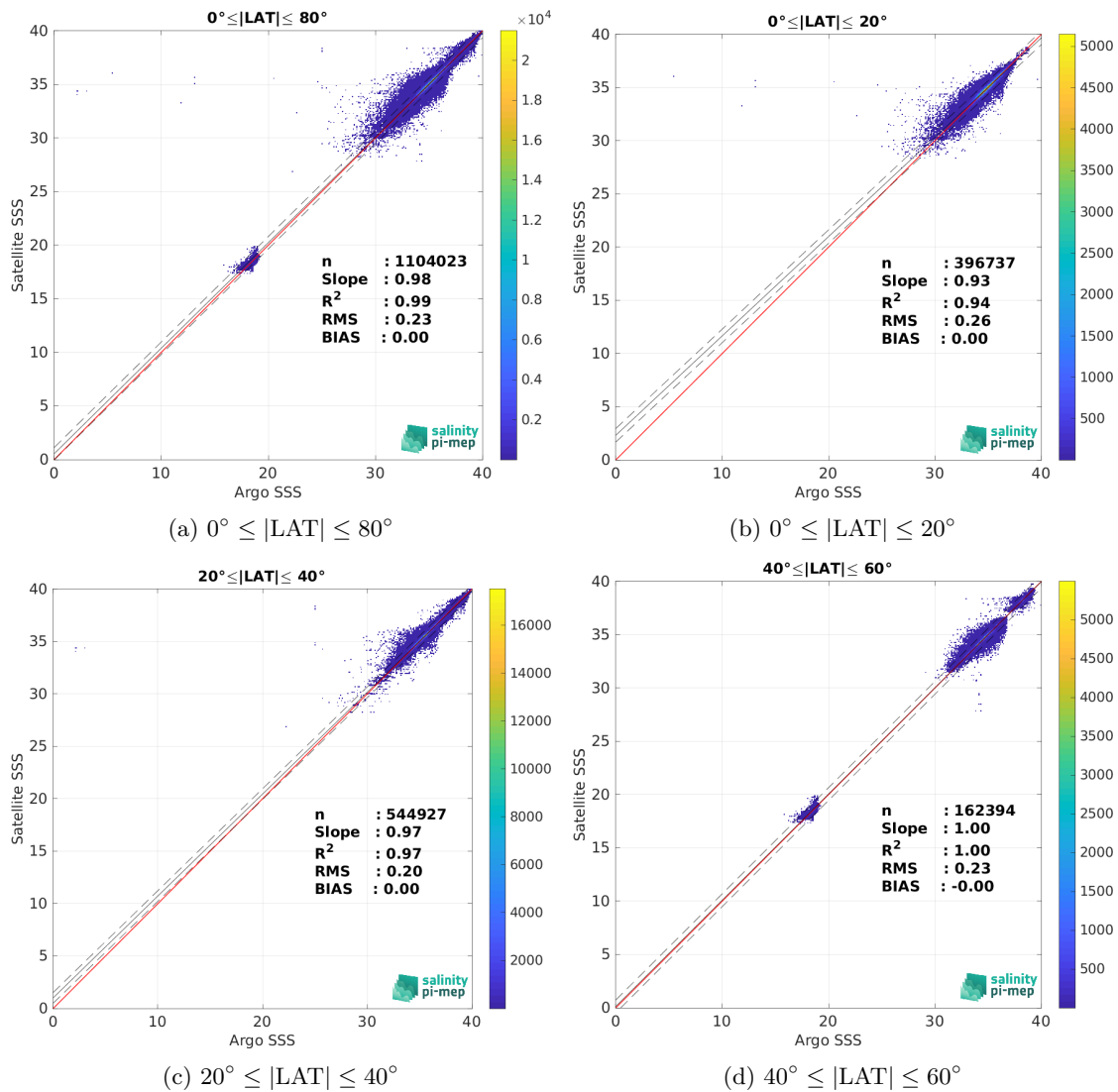
Figure 10: Contour maps of the concentration of ISAS SSS (y-axis) versus Argo SSS (x-axis) at match-up pairs for different latitude bands. For each plot, the red line shows x=y . The black thin and dashed lines indicate a linear fit through the data cloud and the \pm 95\% confidence levels, respectively. The number match-up pairs n , the slope and R^2 coefficient of the linear fit, the root mean square (RMS) and the mean bias between satellite and in situ data are indicated for each latitude band in each plots.
