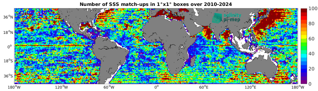
Figure 5: Number of SSS match-ups between Argo SSS and the ISAS SSS product for the Mid-Low Latitudes 45N-45S Pi-MEP region over 1^\circ \times 1^\circ boxes and for the full satellite product period.
