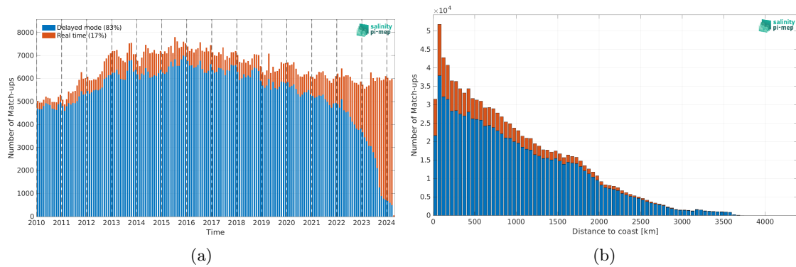
Figure 2: Number of match-ups between Argo and ISAS SSS as a function of time (a) and as function of the distance to coast (b) over the Mid-Low Latitudes 45N-45S Pi-MEP region and for the full satellite product period.
