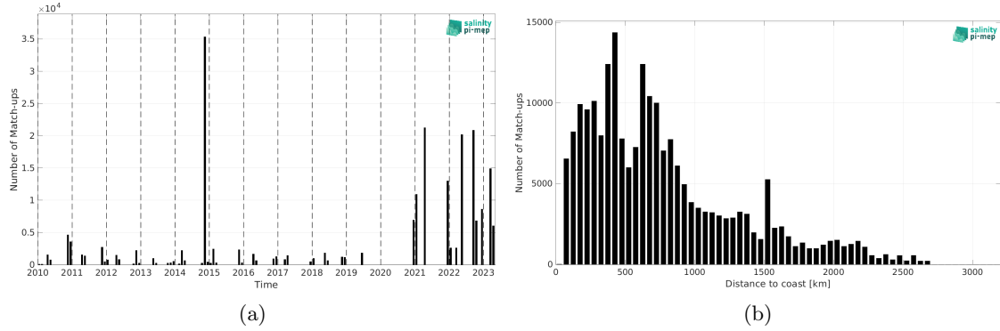
Figure 2: Number of match-ups between TSG (Polarstern) and CCI SSS L4 Merged-OI v5.5 - 7-day running (ESA) SSS as a function of time (a) and as function of the distance to coast (b) over the Mid-Low Latitudes 45N-45S Pi-MEP region and for the full satellite product period.
