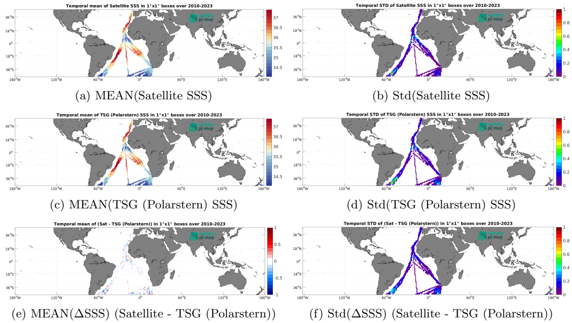
Figure 7: Temporal mean (left) and Std (right) of SSS from CCI SSS L4 Merged-OI v5.5 - 7-day running (ESA) (top), TSG (Polarstern) (middle), and of \Delta SSS (Satellite - TSG (Polarstern)). Only match-up pairs are used to generate these maps.
