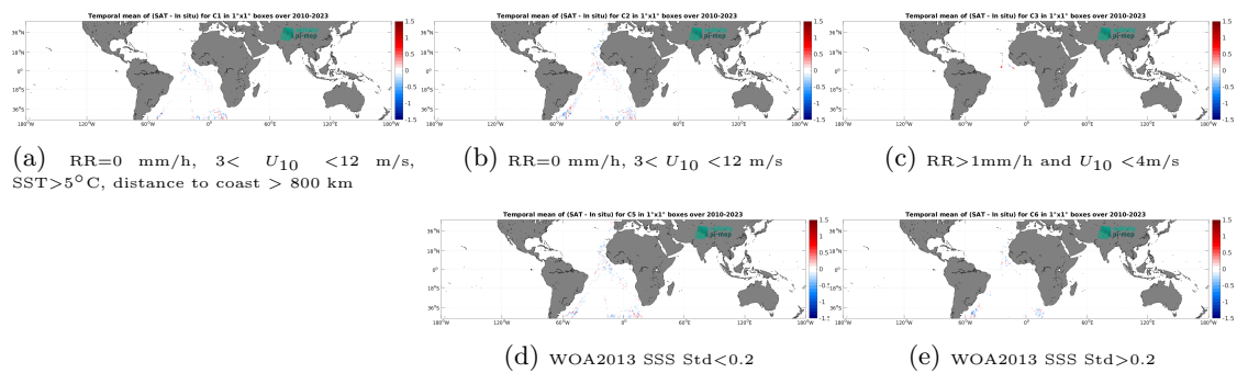
Figure 14: Temporal mean gridded over spatial boxes of size 1^\circ \times 1^\circ of \Delta SSS (CCI SSS L4 Merged-OI v5.5 - 7-day running (ESA) - TSG (Polarstern)) for 5 different subdatasets corresponding to:RR=0 mm/h, 3 < U_{10} < 12 m/s, SST > 5°C, distance to coast > 800 km (a), RR=0 mm/h, 3 < U_{10} < 12 m/s (b), RR > 1mm/h and U_{10} < 4 m/s (c), WOA2013 SSS Std < 0.2 (d), WOA2013 SSS Std > 0.2 (e).
