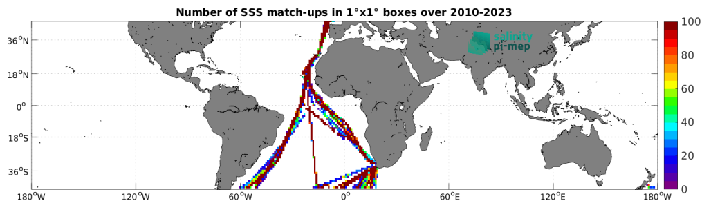
Figure 5: Number of SSS match-ups between TSG (Polarstern) SSS and the CCI SSS L4 Merged-OI v5.5 - 7-day running (ESA) SSS product for the Mid-Low Latitudes 45N-45S Pi-MEP region over 1^\circ \times 1^\circ boxes and for the full satellite product period.
