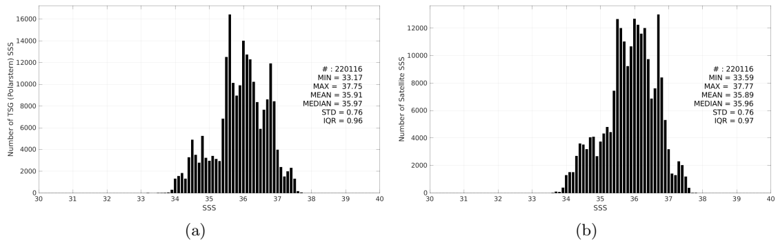
Figure 3: Histograms of SSS from TSG (Polarstern) (a) and CCI SSS L4 Merged-OI v5.5 - 7-day running (ESA) (b) considering all match-up pairs per bins of 0.1 over the Mid-Low Latitudes 45N-45S Pi-MEP region and for the full satellite product period.
