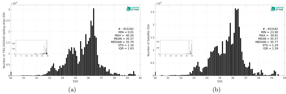
Figure 3: Histograms of SSS from TSG (GOSUD-Sailing-ship) (a) and CCI SSS L4 Merged-OI v5.5 - 7-day running (ESA) (b) considering all match-up pairs per bins of 0.1 over the Mid-Low Latitudes 45N-45S Pi-MEP region and for the full satellite product period.
