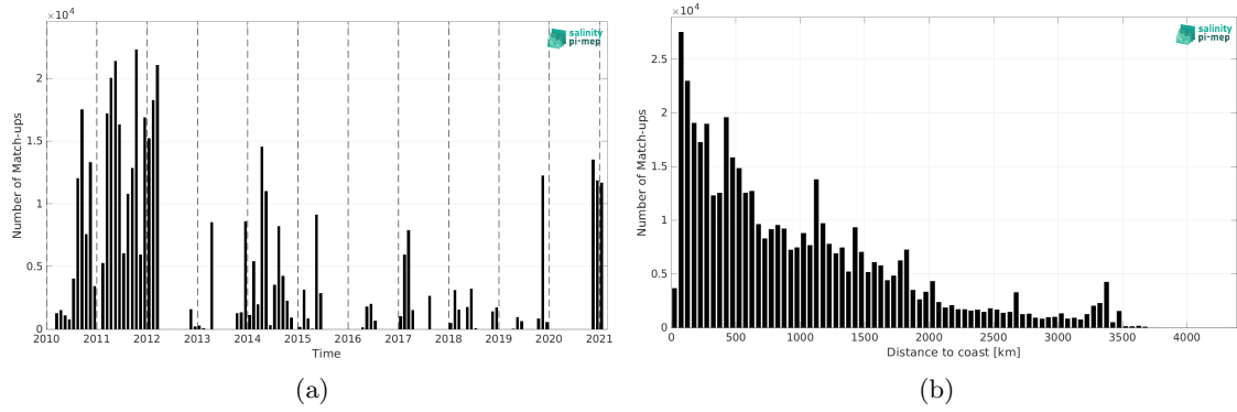
Figure 2: Number of match-ups between TSG (GOSUD-Sailing-ship) and CCI SSS L4 Merged-OI v5.5 - 7-day running (ESA) SSS as a function of time (a) and as function of the distance to coast (b) over the Mid-Low Latitudes 45N-45S Pi-MEP region and for the full satellite product period.
