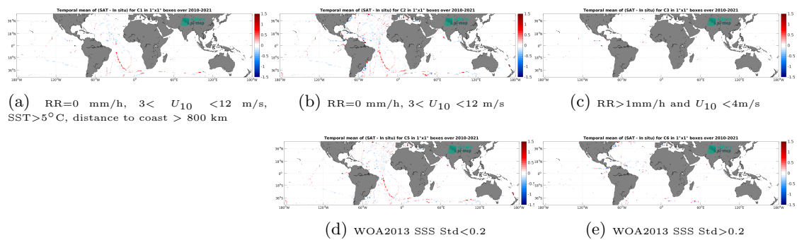
Figure 14: Temporal mean gridded over spatial boxes of size 1^\circ \times 1^\circ of \Delta SSS (CCI SSS L4 Merged-OI v5.5 - 7-day running (ESA) - TSG (GOSUD-Sailing-ship)) for 5 different subdatasets corresponding to: RR=0 mm/h, 3 < U_{10} < 12 m/s, SST > 5^\circ\text{C} , distance to coast > 800 km (a), RR=0 mm/h, 3 < U_{10} < 12 m/s (b), RR > 1 mm/h and U_{10} < 4 m/s (c), WOA2013 SSS Std < 0.2 (d), WOA2013 SSS Std > 0.2 (e).
