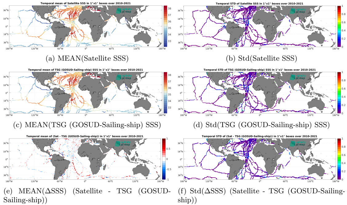
Figure 7: Temporal mean (left) and Std (right) of SSS from CCI SSS L4 Merged-OI v5.5 - 7-day running (ESA) (top), TSG (GOSUD-Sailing-ship) (middle), and of \Delta SSS (Satellite - TSG (GOSUD-Sailing-ship)). Only match-up pairs are used to generate these maps.
