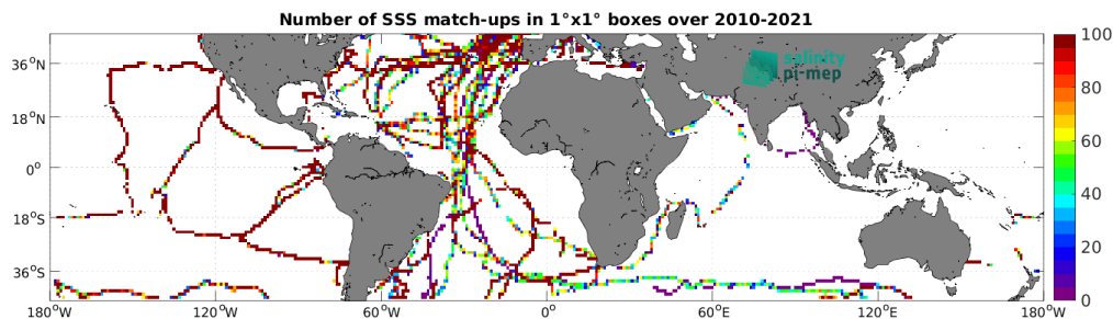
Figure 5: Number of SSS match-ups between TSG (GOSUD-Sailing-ship) SSS and the CCI SSS L4 Merged-OI v5.5 - 7-day running (ESA) SSS product for the Mid-Low Latitudes 45N-45S Pi-MEP region over 1^\circ \times 1^\circ boxes and for the full satellite product period.
