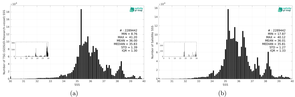
Figure 3: Histograms of SSS from TSG (GOSUD-Research-vessel) (a) and CCI SSS L4 Merged-OI v5.5 - 7-day running (ESA) (b) considering all match-up pairs per bins of 0.1 over the Mid-Low Latitudes 45N-45S Pi-MEP region and for the full satellite product period.
