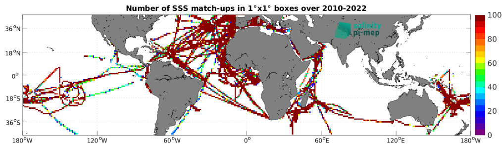
Figure 5: Number of SSS match-ups between TSG (GOSUD-Research-vessel) SSS and the CCI SSS L4 Merged-OI v5.5 - 7-day running (ESA) SSS product for the Mid-Low Latitudes 45N-45S Pi-MEP region over 1^\circ \times 1^\circ boxes and for the full satellite product period.
