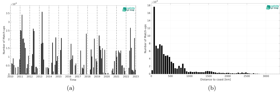
Figure 2: Number of match-ups between TSG (CSIC-UTM) and CCI SSS L4 Merged-OI v5.5 - 7-day running (ESA) SSS as a function of time (a) and as function of the distance to coast (b) over the Mid-Low Latitudes 45N-45S Pi-MEP region and for the full satellite product period.
