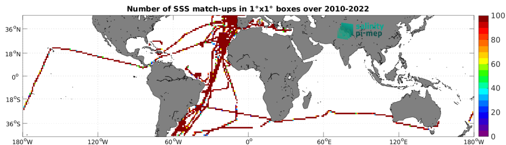
Figure 5: Number of SSS match-ups between TSG (CSIC-UTM) SSS and the CCI SSS L4 Merged-OI v5.5 - 7-day running (ESA) SSS product for the Mid-Low Latitudes 45N-45S Pi-MEP region over 1^\circ \times 1^\circ boxes and for the full satellite product period.
