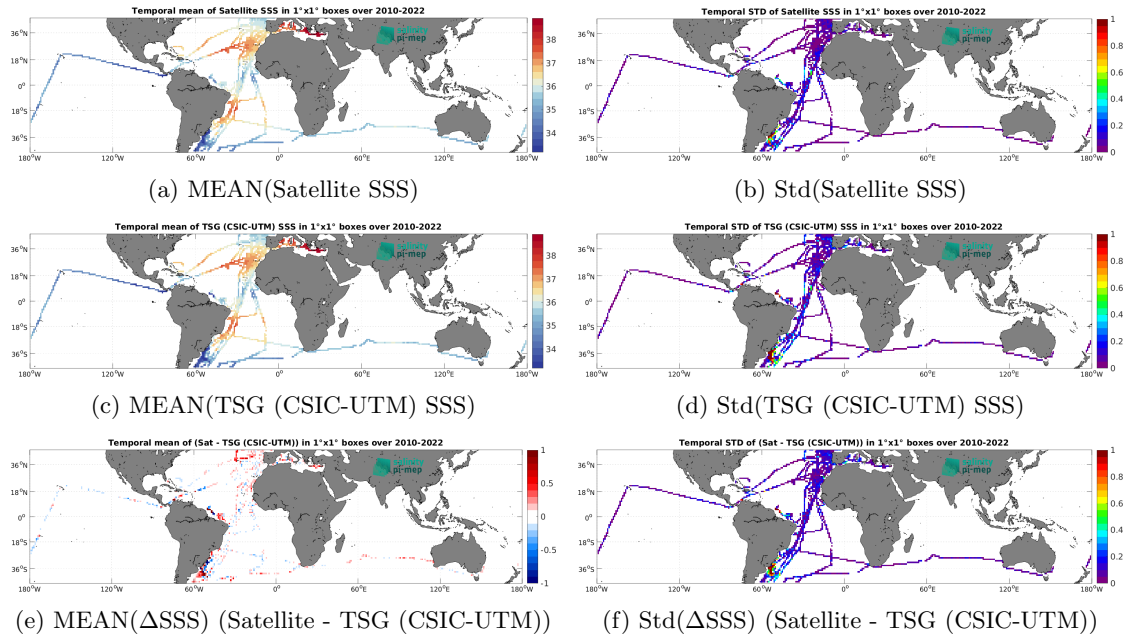
Figure 7: Temporal mean (left) and Std (right) of SSS from CCI SSS L4 Merged-OI v5.5 - 7-day running (ESA) (top), TSG (CSIC-UTM) (middle), and of \Delta SSS (Satellite - TSG (CSIC-UTM)). Only match-up pairs are used to generate these maps.
