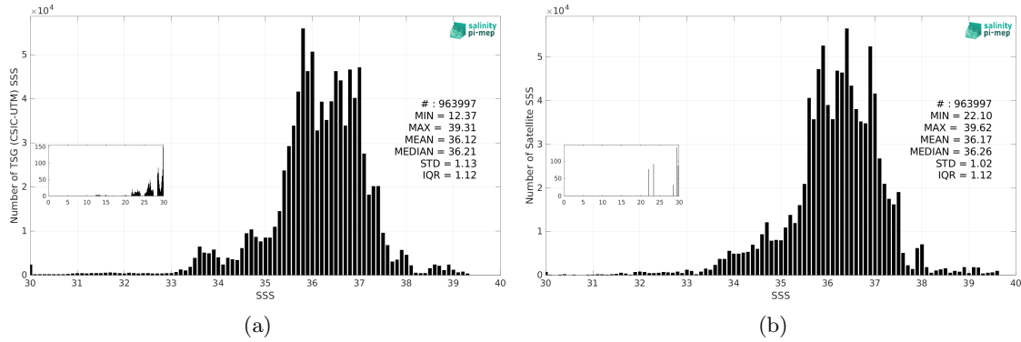
Figure 3: Histograms of SSS from TSG (CSIC-UTM) (a) and CCI SSS L4 Merged-OI v5.5 - 7-day running (ESA) (b) considering all match-up pairs per bins of 0.1 over the Mid-Low Latitudes 45N-45S Pi-MEP region and for the full satellite product period.
