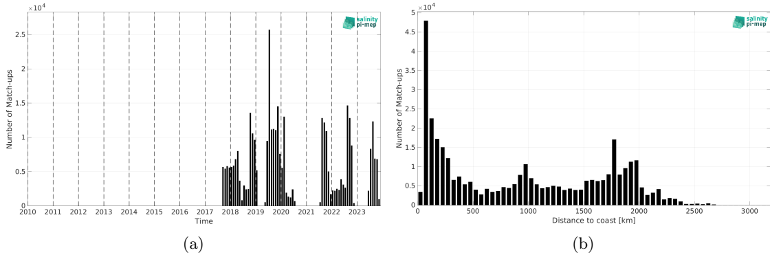
Figure 2: Number of match-ups between Saildrone and CCI SSS L4 Merged-OI v5.5 - 7-day running (ESA) SSS as a function of time (a) and as function of the distance to coast (b) over the Mid-Low Latitudes 45N-45S Pi-MEP region and for the full satellite product period.
