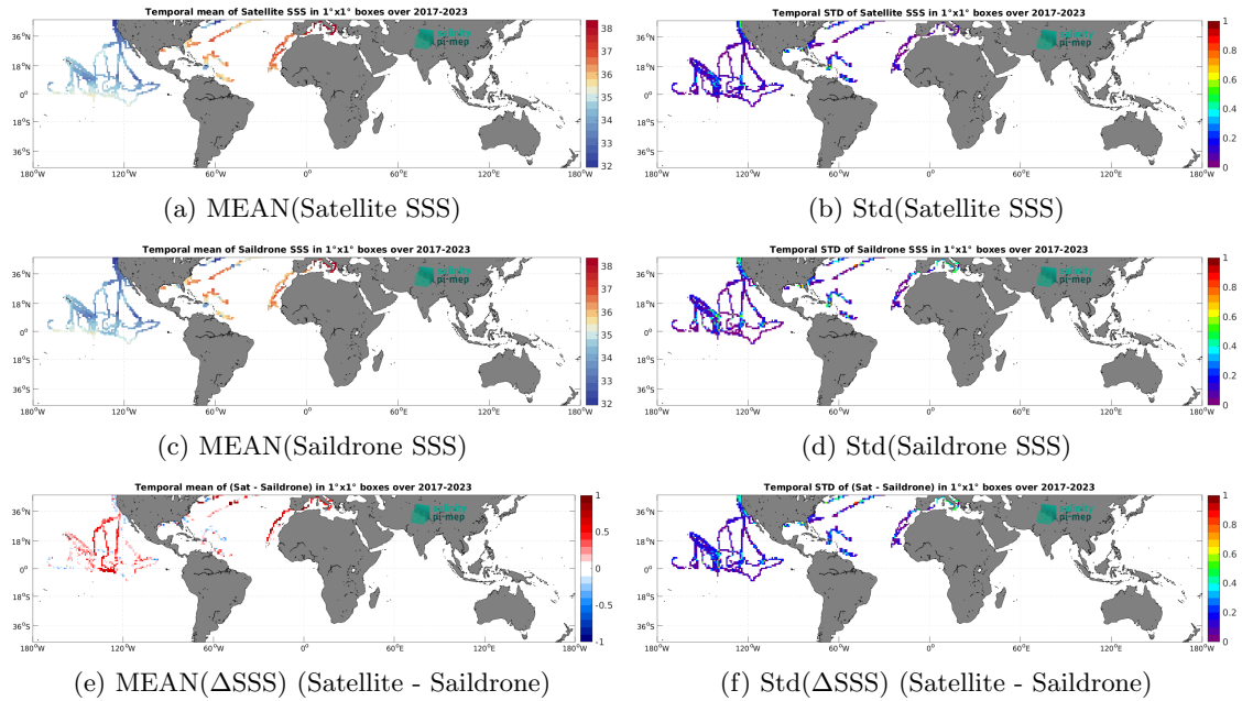
Figure 7: Temporal mean (left) and Std (right) of SSS from CCI SSS L4 Merged-OI v5.5 - 7-day running (ESA) (top), Saildrone (middle), and of \Delta SSS (Satellite - Saildrone). Only match-up pairs are used to generate these maps.
