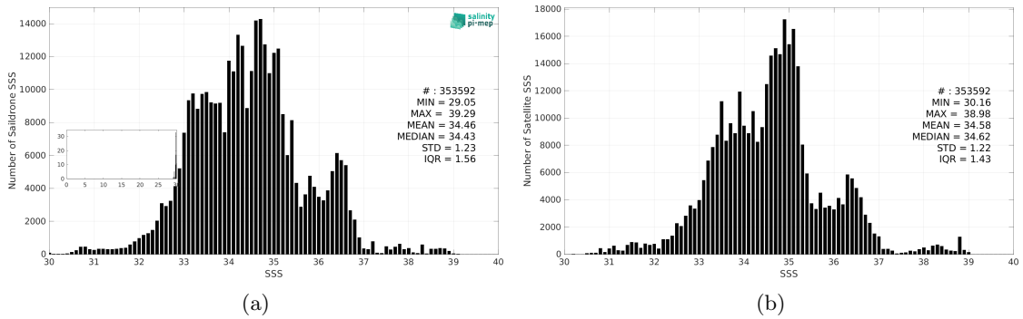
Figure 3: Histograms of SSS from Saildrone (a) and CCI SSS L4 Merged-OI v5.5 - 7-day running (ESA) (b) considering all match-up pairs per bins of 0.1 over the Mid-Low Latitudes 45N-45S Pi-MEP region and for the full satellite product period.
