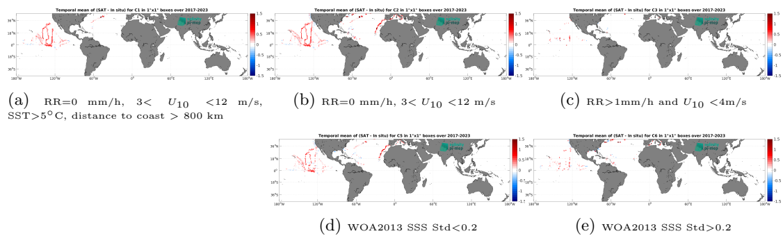
Figure 14: Temporal mean gridded over spatial boxes of size 1^\circ \times 1^\circ of \Delta SSS (CCI SSS L4 Merged-OI v5.5 - 7-day running (ESA) - Saildrone) for 5 different subdatasets corresponding to:RR=0 mm/h, 3 < U_{10} < 12 m/s, SST >5^\circ C, distance to coast > 800 km (a), RR=0 mm/h, 3 < U_{10} < 12 m/s (b), RR >1 mm/h and U_{10} < 4 m/s (c), WOA2013 SSS Std <0.2 (d), WOA2013 SSS Std >0.2 (e).
