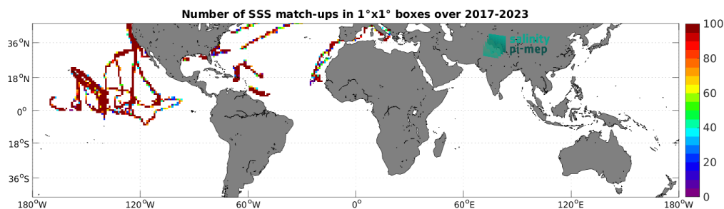
Figure 5: Number of SSS match-ups between Saildrone SSS and the CCI SSS L4 Merged-OI v5.5 - 7-day running (ESA) SSS product for the Mid-Low Latitudes 45N-45S Pi-MEP region over 1^\circ \times 1^\circ boxes and for the full satellite product period.
