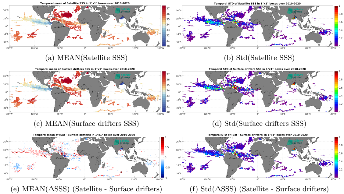
Figure 6: Temporal mean (left) and Std (right) of SSS from CCI SSS L4 Merged-OI v5.5 - 7-day running (ESA) (top), Surface drifters (middle), and of \Delta SSS (Satellite - Surface drifters). Only match-up pairs are used to generate these maps.
