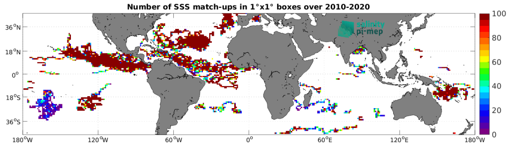
Figure 4: Number of SSS match-ups between Surface drifters SSS and the CCI SSS L4 Merged-OI v5.5 - 7-day running (ESA) SSS product for the Mid-Low Latitudes 45N-45S Pi-MEP region over 1^\circ \times 1^\circ boxes and for the full satellite product period.
