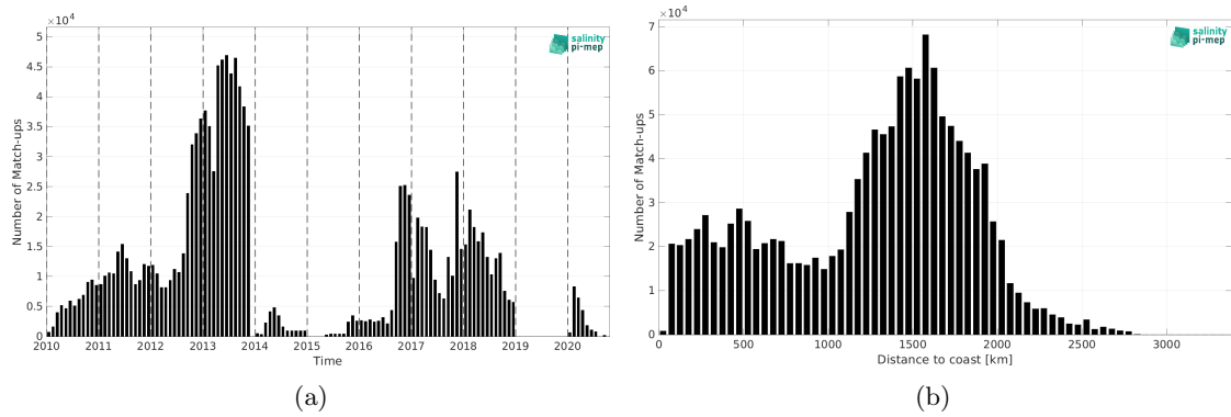
Figure 2: Number of match-ups between Surface drifters and CCI SSS L4 Merged-OI v5.5 - 7-day running (ESA) SSS as a function of time (a) and as function of the distance to coast (b) over the Mid-Low Latitudes 45N-45S Pi-MEP region and for the full satellite product period.
