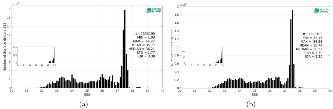
Figure 3: Histograms of SSS from Surface drifters (a) and CCI SSS L4 Merged-OI v5.5 - 7-day running (ESA) (b) considering all match-up pairs per bins of 0.1 over the Mid-Low Latitudes 45N-45S Pi-MEP region and for the full satellite product period.
