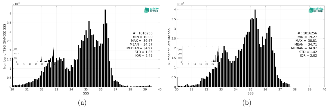
Figure 3: Histograms of SSS from TSG (SAMOS) (a) and CCI SSS L4 Merged-OI v5.5 - 30-day running (ESA) (b) considering all match-up pairs per bins of 0.1 over the Mid-Low Latitudes 45N-45S Pi-MEP region and for the full satellite product period.
