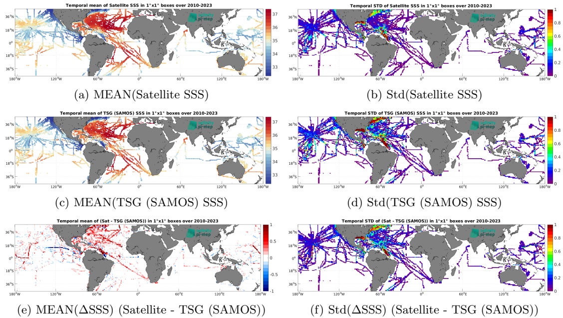
Figure 7: Temporal mean (left) and Std (right) of SSS from CCI SSS L4 Merged-OI v5.5 - 30-day running (ESA) (top), TSG (SAMOS) (middle), and of \Delta SSS (Satellite - TSG (SAMOS)). Only match-up pairs are used to generate these maps.
