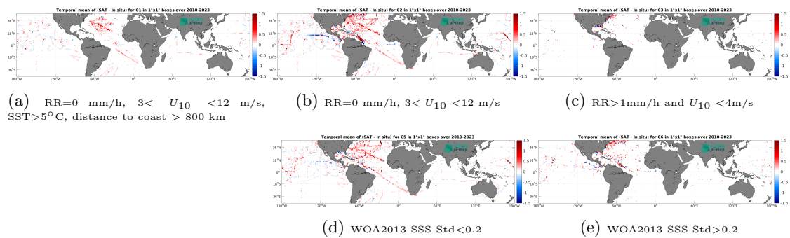
Figure 14: Temporal mean gridded over spatial boxes of size 1^\circ \times 1^\circ of \Delta\text{SSS} (CCI SSS L4 Merged-OI v5.5 - 30-day running (ESA) - TSG (SAMOS)) for 5 different subdatasets corresponding to:RR=0 mm/h, 3 < U_{10} < 12 m/s, SST >5^\circ\text{C} , distance to coast > 800 km (a), RR=0 mm/h, 3 < U_{10} < 12 m/s (b), RR >1 mm/h and U_{10} < 4 m/s (c), WOA2013 SSS Std <0.2 (d), WOA2013 SSS Std >0.2 (e).
