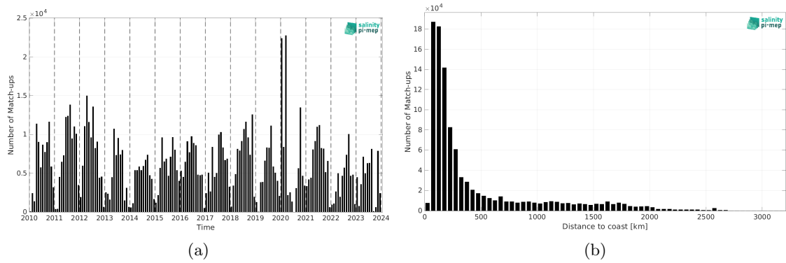
Figure 2: Number of match-ups between TSG (SAMOS) and CCI SSS L4 Merged-OI v5.5 - 30-day running (ESA) SSS as a function of time (a) and as function of the distance to coast (b) over the Mid-Low Latitudes 45N-45S Pi-MEP region and for the full satellite product period.
