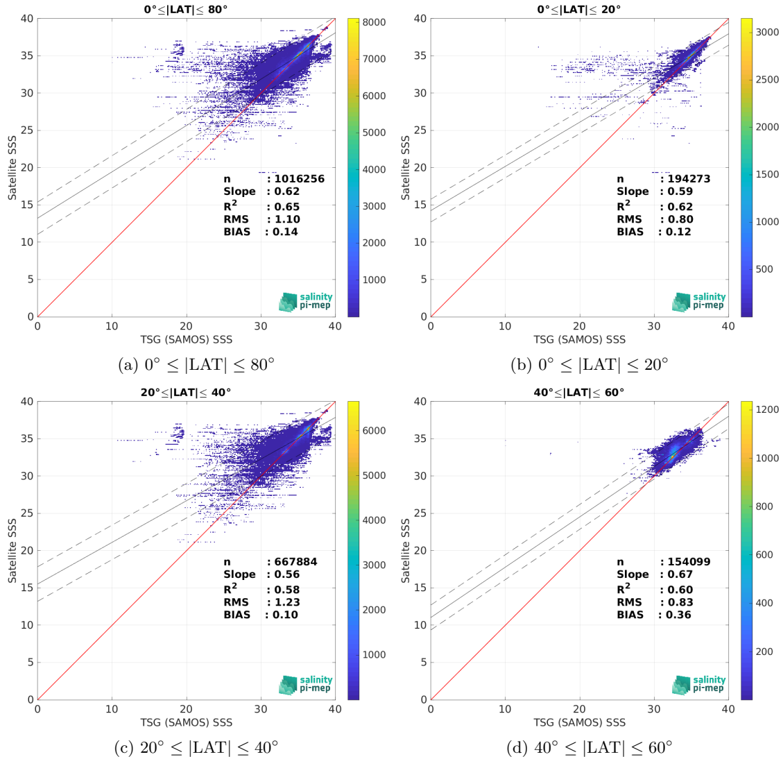
Figure 10: Contour maps of the concentration of CCI SSS L4 Merged-OI v5.5 - 30-day running (ESA) SSS (y-axis) versus TSG (SAMOS) SSS (x-axis) at match-up pairs for different latitude bands. For each plot, the red line shows x=y . The black thin and dashed lines indicate a linear fit through the data cloud and the \pm 95\% confidence levels, respectively. The number match-up pairs n , the slope and R^2 coefficient of the linear fit, the root mean square (RMS) and the mean bias between satellite and in situ data are indicated for each latitude band in each plots.
