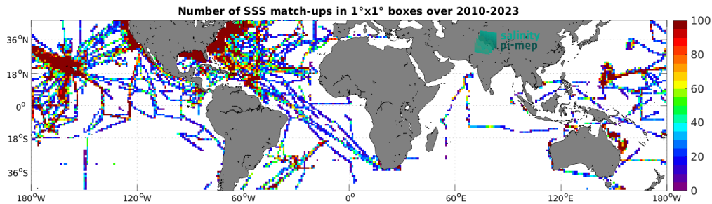
Figure 5: Number of SSS match-ups between TSG (SAMOS) SSS and the CCI SSS L4 Merged-OI v5.5 - 30-day running (ESA) SSS product for the Mid-Low Latitudes 45N-45S Pi-MEP region over 1^\circ \times 1^\circ boxes and for the full satellite product period.
