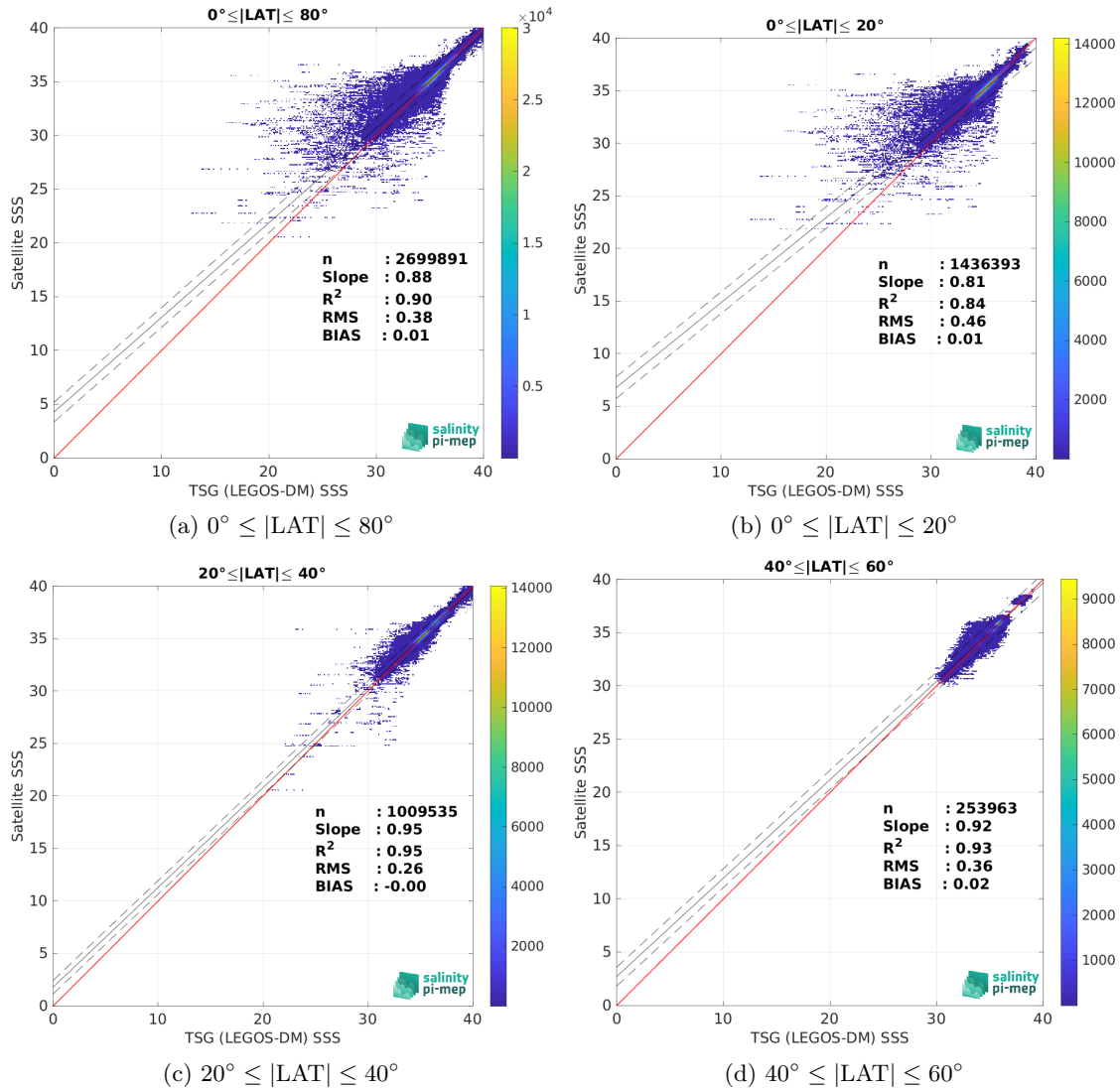
Figure 10: Contour maps of the concentration of CCI SSS L4 Merged-OI v5.5 - 30-day running (ESA) SSS (y-axis) versus TSG (LEGOS-DM) SSS (x-axis) at match-up pairs for different latitude bands. For each plot, the red line shows x=y . The black thin and dashed lines indicate a linear fit through the data cloud and the \pm 95\% confidence levels, respectively. The number match-up pairs n , the slope and R^2 coefficient of the linear fit, the root mean square (RMS) and the mean bias between satellite and in situ data are indicated for each latitude band in each plots.
