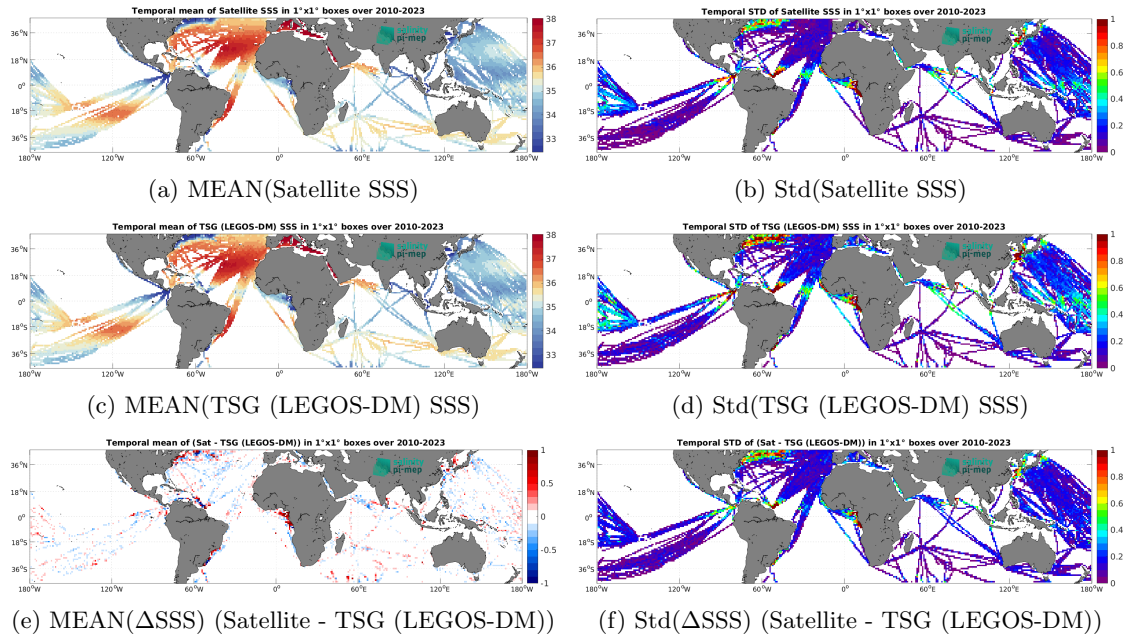
Figure 7: Temporal mean (left) and Std (right) of SSS from CCI SSS L4 Merged-OI v5.5 - 30-day running (ESA) (top), TSG (LEGOS-DM) (middle), and of \Delta SSS (Satellite - TSG (LEGOS-DM)). Only match-up pairs are used to generate these maps.
