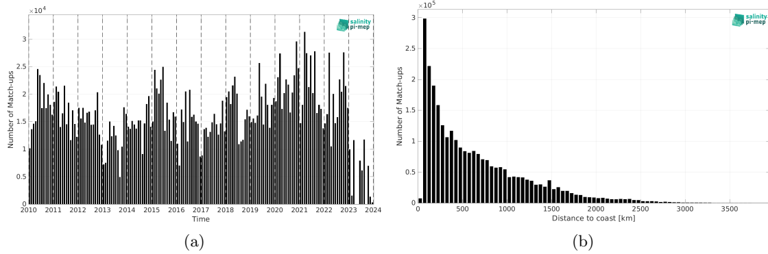
Figure 2: Number of match-ups between TSG (LEGOS-DM) and CCI SSS L4 Merged-OI v5.5 - 30-day running (ESA) SSS as a function of time (a) and as function of the distance to coast (b) over the Mid-Low Latitudes 45N-45S Pi-MEP region and for the full satellite product period.
