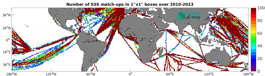
Figure 5: Number of SSS match-ups between TSG (LEGOS-DM) SSS and the CCI SSS L4 Merged-OI v5.5 - 30-day running (ESA) SSS product for the Mid-Low Latitudes 45N-45S Pi-MEP region over 1^\circ \times 1^\circ boxes and for the full satellite product period.
