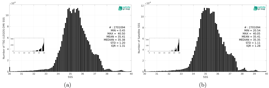
Figure 3: Histograms of SSS from TSG (LEGOS-DM) (a) and CCI SSS L4 Merged-OI v5.5 - 30-day running (ESA) (b) considering all match-up pairs per bins of 0.1 over the Mid-Low Latitudes 45N-45S Pi-MEP region and for the full satellite product period.
