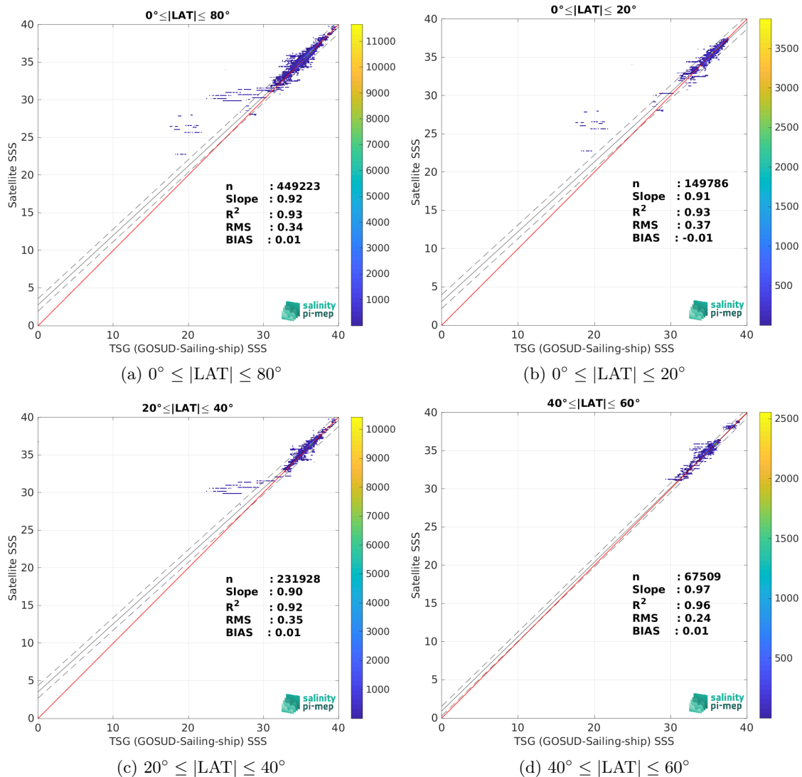
Figure 10: Contour maps of the concentration of CCI SSS L4 Merged-OI v5.5 - 30-day running (ESA) SSS (y-axis) versus TSG (GOSUD-Sailing-ship) SSS (x-axis) at match-up pairs for different latitude bands. For each plot, the red line shows x=y . The black thin and dashed lines indicate a linear fit through the data cloud and the \pm 95\% confidence levels, respectively. The number match-up pairs n , the slope and R^2 coefficient of the linear fit, the root mean square (RMS) and the mean bias between satellite and in situ data are indicated for each latitude band in each plots.
