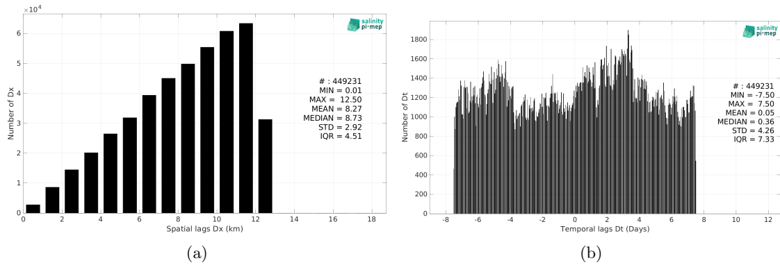
Figure 6: Histograms of the spatial (a) and temporal (b) lags between the location/time of the TSG (GOSUD-Sailing-ship) measurement and the date of the corresponding CCI SSS L4 Merged-OI v5.5 - 30-day running (ESA) SSS pixel.
