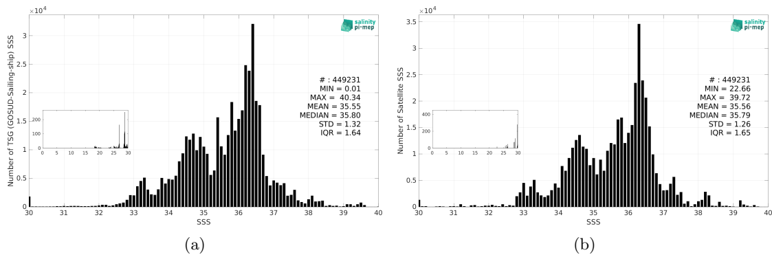
Figure 3: Histograms of SSS from TSG (GOSUD-Sailing-ship) (a) and CCI SSS L4 Merged-OI v5.5 - 30-day running (ESA) (b) considering all match-up pairs per bins of 0.1 over the Mid-Low Latitudes 45N-45S Pi-MEP region and for the full satellite product period.
