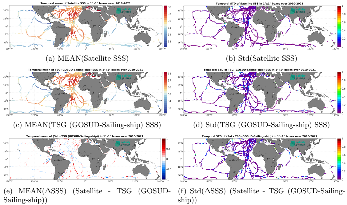
Figure 7: Temporal mean (left) and Std (right) of SSS from CCI SSS L4 Merged-OI v5.5 - 30-day running (ESA) (top), TSG (GOSUD-Sailing-ship) (middle), and of \Delta SSS (Satellite - TSG (GOSUD-Sailing-ship)). Only match-up pairs are used to generate these maps.
