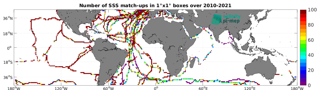
Figure 5: Number of SSS match-ups between TSG (GOSUD-Sailing-ship) SSS and the CCI SSS L4 Merged-OI v5.5 - 30-day running (ESA) SSS product for the Mid-Low Latitudes 45N-45S Pi-MEP region over 1^\circ \times 1^\circ boxes and for the full satellite product period.
