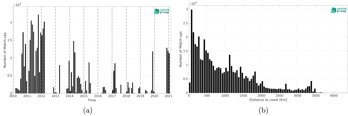
Figure 2: Number of match-ups between TSG (GOSUD-Sailing-ship) and CCI SSS L4 Merged-OI v5.5 - 30-day running (ESA) SSS as a function of time (a) and as function of the distance to coast (b) over the Mid-Low Latitudes 45N-45S Pi-MEP region and for the full satellite product period.
