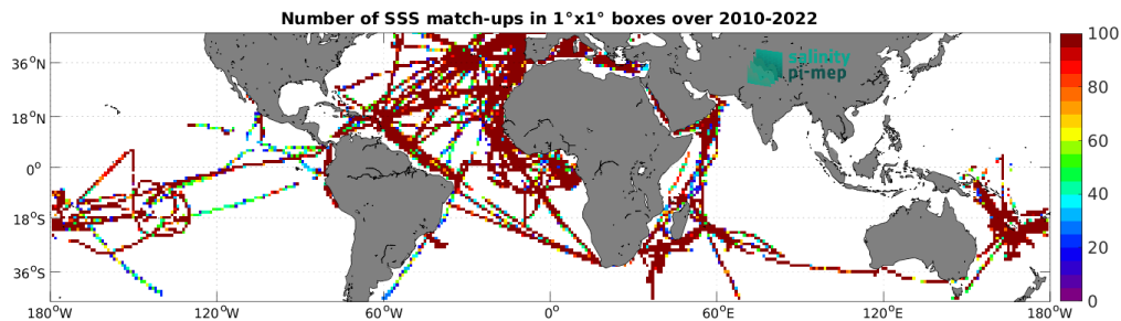
Figure 5: Number of SSS match-ups between TSG (GOSUD-Research-vessel) SSS and the CCI SSS L4 Merged-OI v5.5 - 30-day running (ESA) SSS product for the Mid-Low Latitudes 45N-45S Pi-MEP region over 1^\circ \times 1^\circ boxes and for the full satellite product period.
