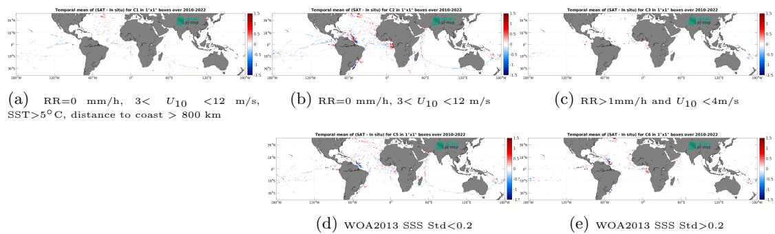
Figure 14: Temporal mean gridded over spatial boxes of size 1^\circ \times 1^\circ of \Delta SSS (CCI SSS L4 Merged-OI v5.5 - 30-day running (ESA) - TSG (GOSUD-Research-vessel)) for 5 different subdatasets corresponding to:RR=0 mm/h, 3 < U_{10} < 12 m/s, SST > 5^\circ\text{C} , distance to coast > 800 km (a), RR=0 mm/h, 3 < U_{10} < 12 m/s (b), RR > 1 mm/h and U_{10} < 4 m/s (c), WOA2013 SSS Std < 0.2 (d), WOA2013 SSS Std > 0.2 (e).
