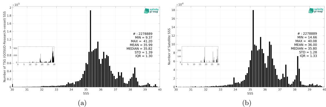
Figure 3: Histograms of SSS from TSG (GOSUD-Research-vessel) (a) and CCI SSS L4 Merged-OI v5.5 - 30-day running (ESA) (b) considering all match-up pairs per bins of 0.1 over the Mid-Low Latitudes 45N-45S Pi-MEP region and for the full satellite product period.
