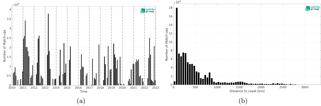
Figure 2: Number of match-ups between TSG (CSIC-UTM) and CCI SSS L4 Merged-OI v5.5 - 30-day running (ESA) SSS as a function of time (a) and as function of the distance to coast (b) over the Mid-Low Latitudes 45N-45S Pi-MEP region and for the full satellite product period.
