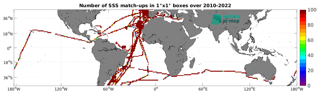
Figure 5: Number of SSS match-ups between TSG (CSIC-UTM) SSS and the CCI SSS L4 Merged-OI v5.5 - 30-day running (ESA) SSS product for the Mid-Low Latitudes 45N-45S Pi-MEP region over 1^\circ \times 1^\circ boxes and for the full satellite product period.
