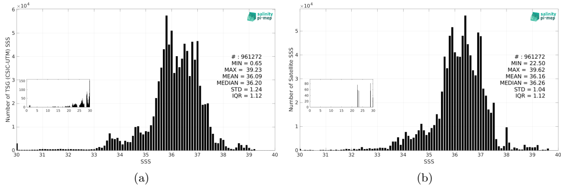
Figure 3: Histograms of SSS from TSG (CSIC-UTM) (a) and CCI SSS L4 Merged-OI v5.5 - 30-day running (ESA) (b) considering all match-up pairs per bins of 0.1 over the Mid-Low Latitudes 45N-45S Pi-MEP region and for the full satellite product period.
