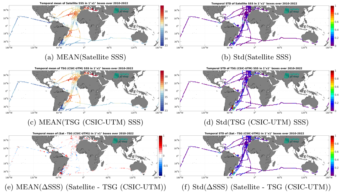
Figure 7: Temporal mean (left) and Std (right) of SSS from CCI SSS L4 Merged-OI v5.5 - 30-day running (ESA) (top), TSG (CSIC-UTM) (middle), and of \Delta SSS (Satellite - TSG (CSIC-UTM)). Only match-up pairs are used to generate these maps.
