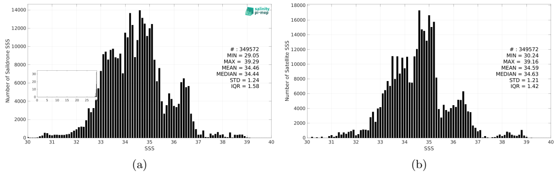
Figure 3: Histograms of SSS from Saildrone (a) and CCI SSS L4 Merged-OI v5.5 - 30-day running (ESA) (b) considering all match-up pairs per bins of 0.1 over the Mid-Low Latitudes 45N-45S Pi-MEP region and for the full satellite product period.
