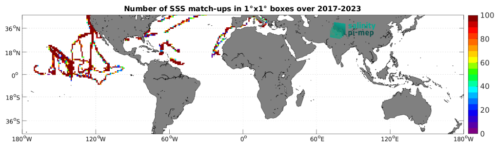
Figure 5: Number of SSS match-ups between Saildrone SSS and the CCI SSS L4 Merged-OI v5.5 - 30-day running (ESA) SSS product for the Mid-Low Latitudes 45N-45S Pi-MEP region over 1^\circ \times 1^\circ boxes and for the full satellite product period.
