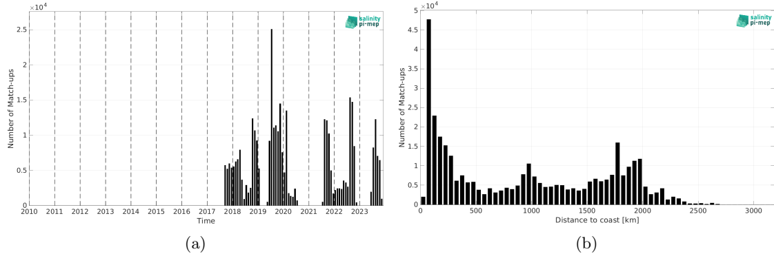
Figure 2: Number of match-ups between Saildrone and CCI SSS L4 Merged-OI v5.5 - 30-day running (ESA) SSS as a function of time (a) and as function of the distance to coast (b) over the Mid-Low Latitudes 45N-45S Pi-MEP region and for the full satellite product period.
