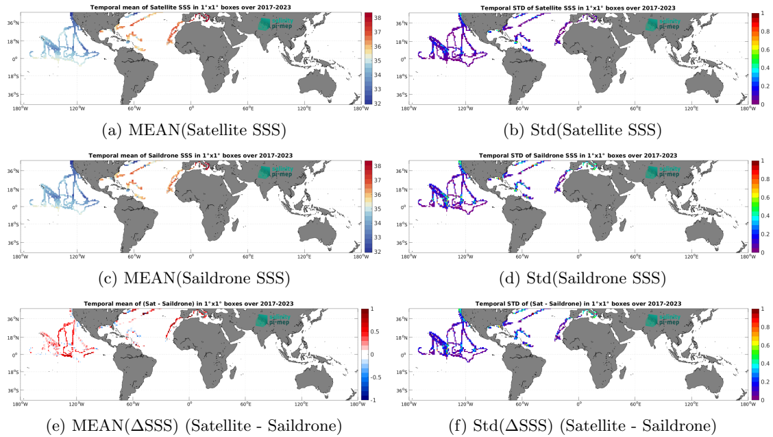
Figure 7: Temporal mean (left) and Std (right) of SSS from CCI SSS L4 Merged-OI v5.5 - 30-day running (ESA) (top), Saildrone (middle), and of \Delta SSS (Satellite - Saildrone). Only match-up pairs are used to generate these maps.
