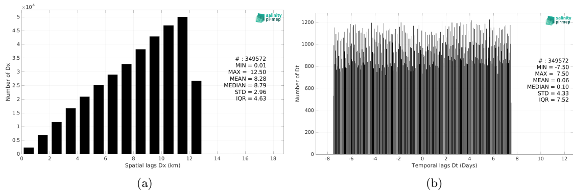
Figure 6: Histograms of the spatial (a) and temporal (b) lags between the location/time of the Sailability measurement and the date of the corresponding CCI SSS L4 Merged-OI v5.5 - 30-day running (ESA) SSS pixel.
