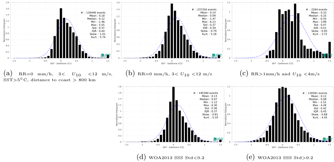
Figure 15: Normalized histogram of \Delta SSS (CCI SSS L4 Merged-OI v5.5 - 30-day running (ESA) - Sailldrone) for 5 different subdatasets corresponding to: RR=0 mm/h, 3 < U_{10} < 12 m/s, SST>5°C, distance to coast > 800 km (a), RR=0 mm/h, 3 < U_{10} < 12 m/s (b), RR>1mm/h and U_{10} < 4 m/s (c), WOA2013 SSS Std<0.2 (d), WOA2013 SSS Std>0.2 (e).
