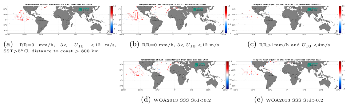
Figure 14: Temporal mean gridded over spatial boxes of size 1^\circ \times 1^\circ of \Delta\text{SSS} (CCI SSS L4 Merged-OI v5.5 - 30-day running (ESA) - Saildrone) for 5 different subdatasets corresponding to: RR=0 mm/h, 3 < U_{10} < 12 m/s, SST > 5°C, distance to coast > 800 km (a), RR=0 mm/h, 3 < U_{10} < 12 m/s (b), RR > 1mm/h and U_{10} < 4 m/s (c), WOA2013 SSS Std < 0.2 (d), WOA2013 SSS Std > 0.2 (e).
