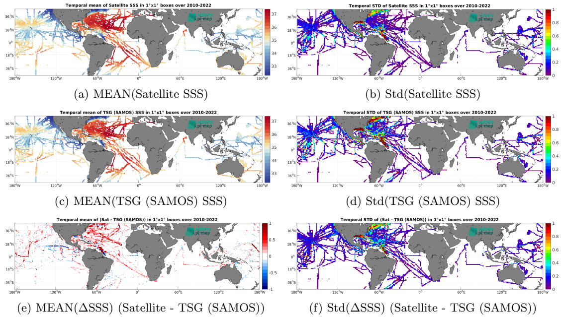
Figure 7: Temporal mean (left) and Std (right) of SSS from CCI SSS L4 Merged-OI v4.41 - 7-day running (ESA) (top), TSG (SAMOS) (middle), and of \Delta SSS (Satellite - TSG (SAMOS)). Only match-up pairs are used to generate these maps.
