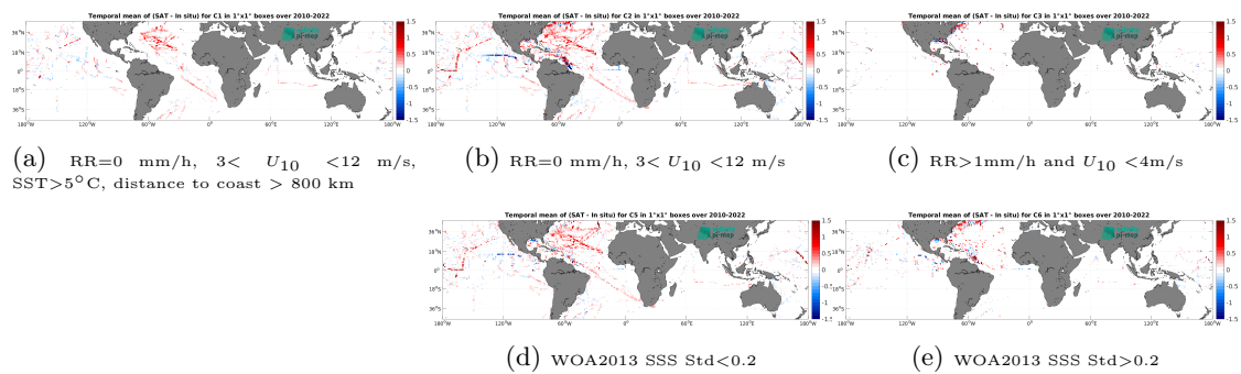
Figure 14: Temporal mean gridded over spatial boxes of size 1^\circ \times 1^\circ of \Delta\text{SSS} (CCI SSS L4 Merged-OI v4.41 - 7-day running (ESA) - TSG (SAMOS)) for 5 different subdatasets corresponding to: RR=0 mm/h, 3 < U_{10} < 12 m/s, SST > 5°C, distance to coast > 800 km (a), RR=0 mm/h, 3 < U_{10} < 12 m/s (b), RR > 1mm/h and U_{10} < 4 m/s (c), WOA2013 SSS Std < 0.2 (d), WOA2013 SSS Std > 0.2 (e).
