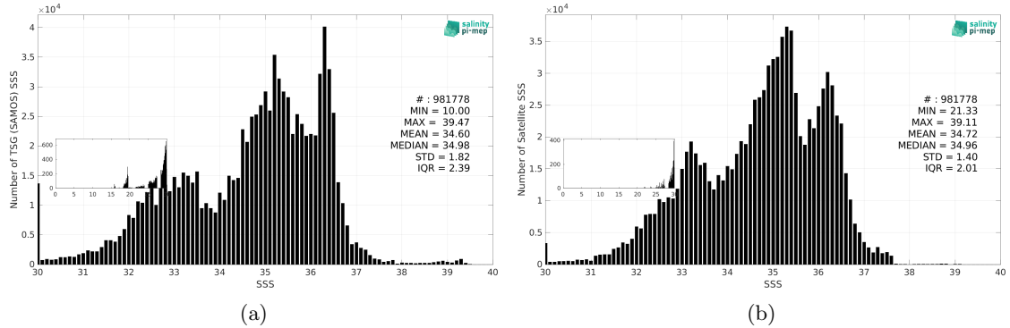
Figure 3: Histograms of SSS from TSG (SAMOS) (a) and CCI SSS L4 Merged-OI v4.41 - 7-day running (ESA) (b) considering all match-up pairs per bins of 0.1 over the Mid-Low Latitudes 45N-45S Pi-MEP region and for the full satellite product period.
