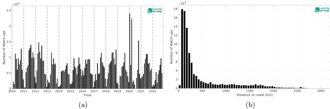
Figure 2: Number of match-ups between TSG (SAMOS) and CCI SSS L4 Merged-OI v4.41 - 7-day running (ESA) SSS as a function of time (a) and as function of the distance to coast (b) over the Mid-Low Latitudes 45N-45S Pi-MEP region and for the full satellite product period.
