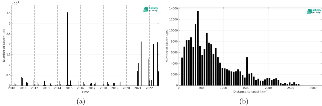
Figure 2: Number of match-ups between TSG (Polarstern) and CCI SSS L4 Merged-OI v4.41 - 7-day running (ESA) SSS as a function of time (a) and as function of the distance to coast (b) over the Mid-Low Latitudes 45N-45S Pi-MEP region and for the full satellite product period.
