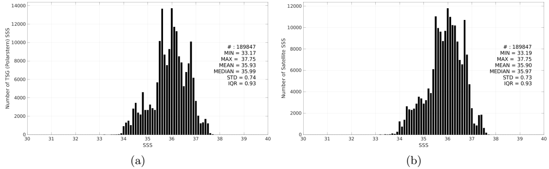
Figure 3: Histograms of SSS from TSG (Polarstern) (a) and CCI SSS L4 Merged-OI v4.41 - 7-day running (ESA) (b) considering all match-up pairs per bins of 0.1 over the Mid-Low Latitudes 45N-45S Pi-MEP region and for the full satellite product period.
