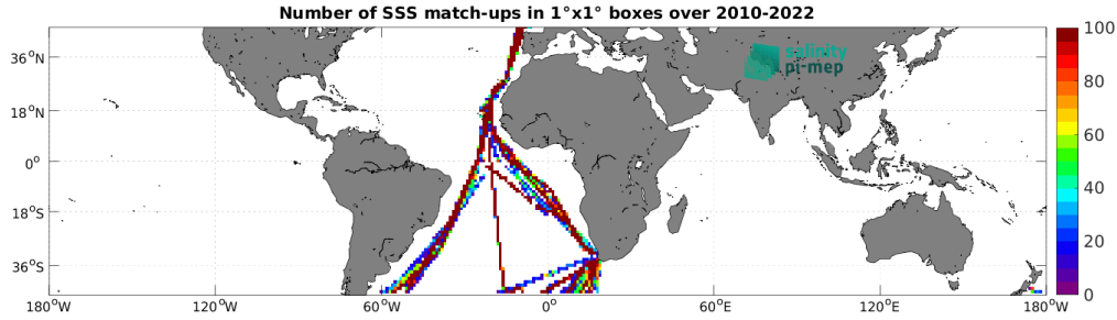
Figure 5: Number of SSS match-ups between TSG (Polarstern) SSS and the CCI SSS L4 Merged-OI v4.41 - 7-day running (ESA) SSS product for the Mid-Low Latitudes 45N-45S Pi-MEP region over 1^\circ \times 1^\circ boxes and for the full satellite product period.
