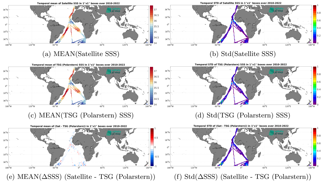
Figure 7: Temporal mean (left) and Std (right) of SSS from CCI SSS L4 Merged-OI v4.41 - 7-day running (ESA) (top), TSG (Polarstern) (middle), and of \Delta SSS (Satellite - TSG (Polarstern)). Only match-up pairs are used to generate these maps.
