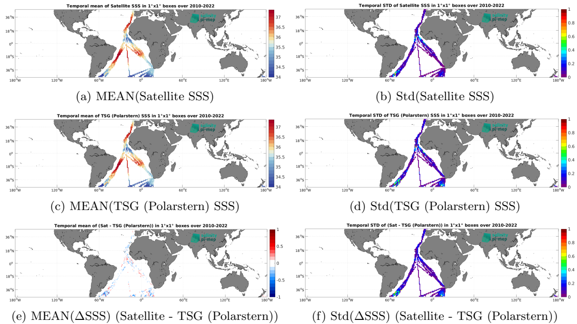
Figure 7: Temporal mean (left) and Std (right) of SSS from CCI SSS L4 Merged-OI v4.41 - 7-day running (ESA) (top), TSG (Polarstern) (middle), and of \Delta SSS (Satellite - TSG (Polarstern)). Only match-up pairs are used to generate these maps.
