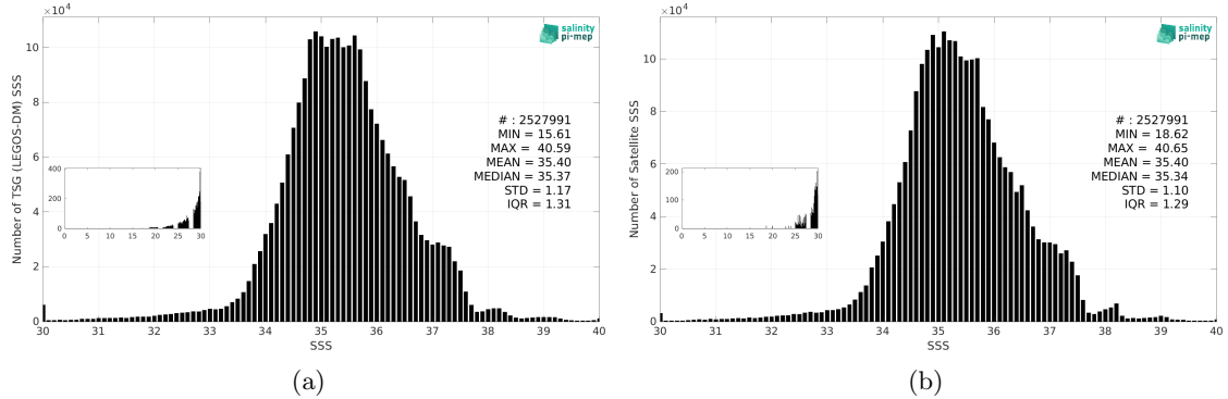
Figure 3: Histograms of SSS from TSG (LEGOS-DM) (a) and CCI SSS L4 Merged-OI v4.41 - 7-day running (ESA) (b) considering all match-up pairs per bins of 0.1 over the Mid-Low Latitudes 45N-45S Pi-MEP region and for the full satellite product period.
