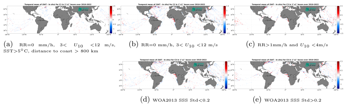
Figure 14: Temporal mean gridded over spatial boxes of size 1^\circ \times 1^\circ of \Delta SSS (CCI SSS L4 Merged-OI v4.41 - 7-day running (ESA) - TSG (LEGOS-DM)) for 5 different subdatasets corresponding to:RR=0 mm/h, 3 < U_{10} < 12 m/s, SST >5^\circ C, distance to coast > 800 km (a), RR=0 mm/h, 3 < U_{10} < 12 m/s (b), RR >1 mm/h and U_{10} < 4 m/s (c), WOA2013 SSS Std <0.2 (d), WOA2013 SSS Std >0.2 (e).
