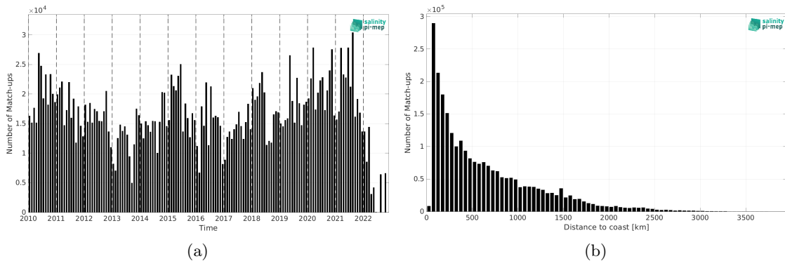
Figure 2: Number of match-ups between TSG (LEGOS-DM) and CCI SSS L4 Merged-OI v4.41 - 7-day running (ESA) SSS as a function of time (a) and as function of the distance to coast (b) over the Mid-Low Latitudes 45N-45S Pi-MEP region and for the full satellite product period.
