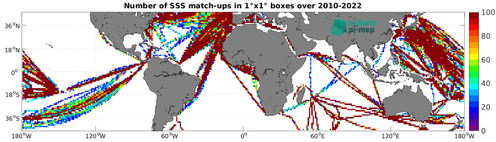
Figure 5: Number of SSS match-ups between TSG (LEGOS-DM) SSS and the CCI SSS L4 Merged-OI v4.41 - 7-day running (ESA) SSS product for the Mid-Low Latitudes 45N-45S Pi-MEP region over 1^\circ \times 1^\circ boxes and for the full satellite product period.
