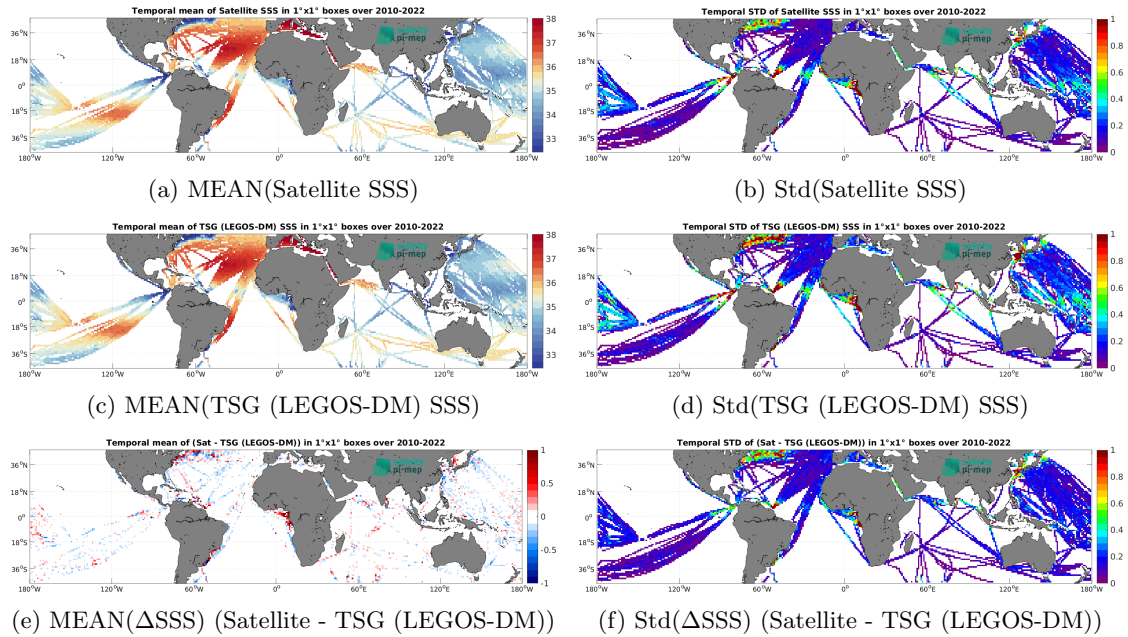
Figure 7: Temporal mean (left) and Std (right) of SSS from CCI SSS L4 Merged-OI v4.41 - 7-day running (ESA) (top), TSG (LEGOS-DM) (middle), and of \Delta SSS (Satellite - TSG (LEGOS-DM)). Only match-up pairs are used to generate these maps.
