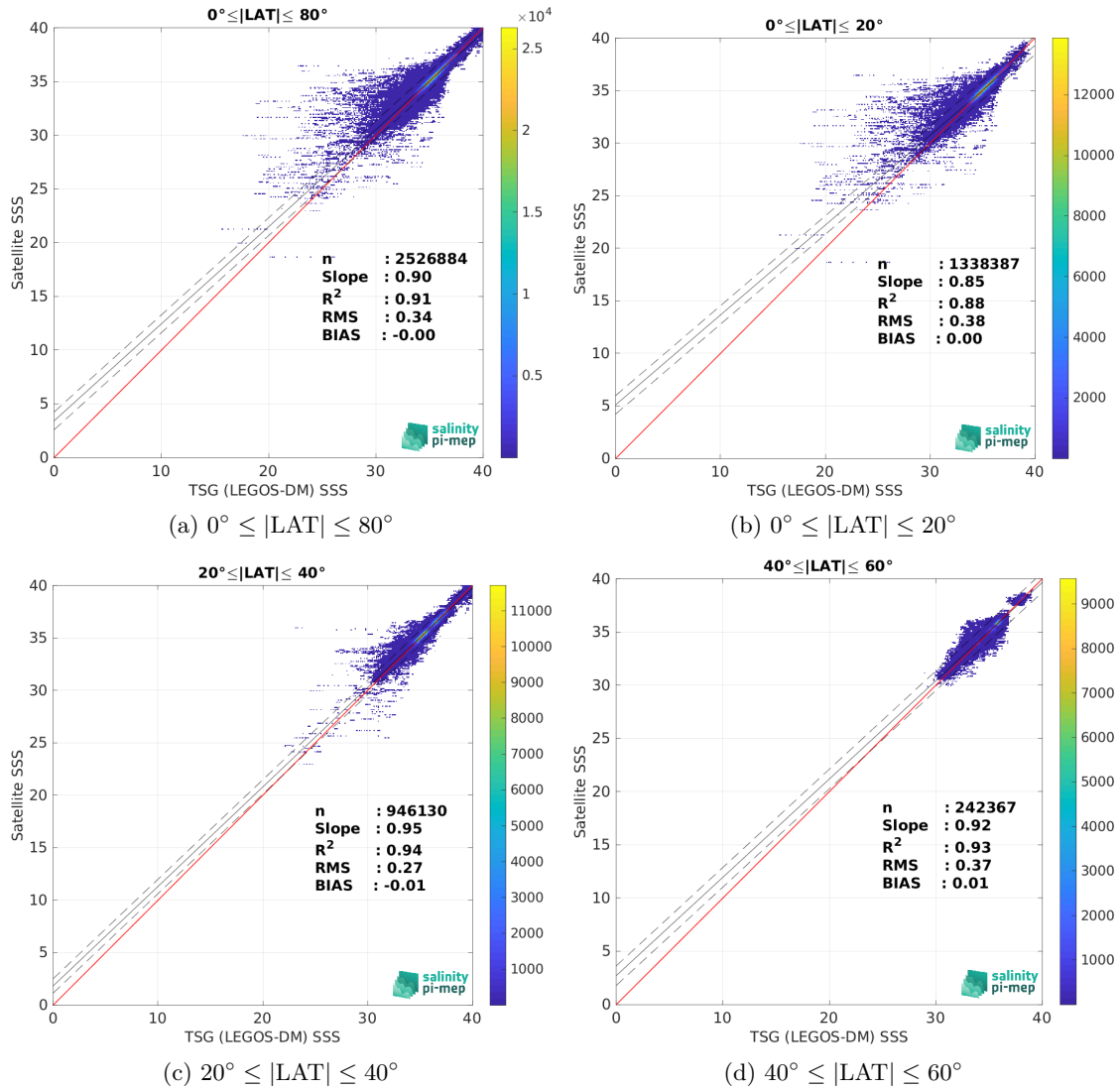
Figure 10: Contour maps of the concentration of CCI SSS L4 Merged-OI v4.41 - 7-day running (ESA) SSS (y-axis) versus TSG (LEGOS-DM) SSS (x-axis) at match-up pairs for different latitude bands. For each plot, the red line shows x=y . The black thin and dashed lines indicate a linear fit through the data cloud and the \pm 95\% confidence levels, respectively. The number match-up pairs n , the slope and R^2 coefficient of the linear fit, the root mean square (RMS) and the mean bias between satellite and in situ data are indicated for each latitude band in each plots.
