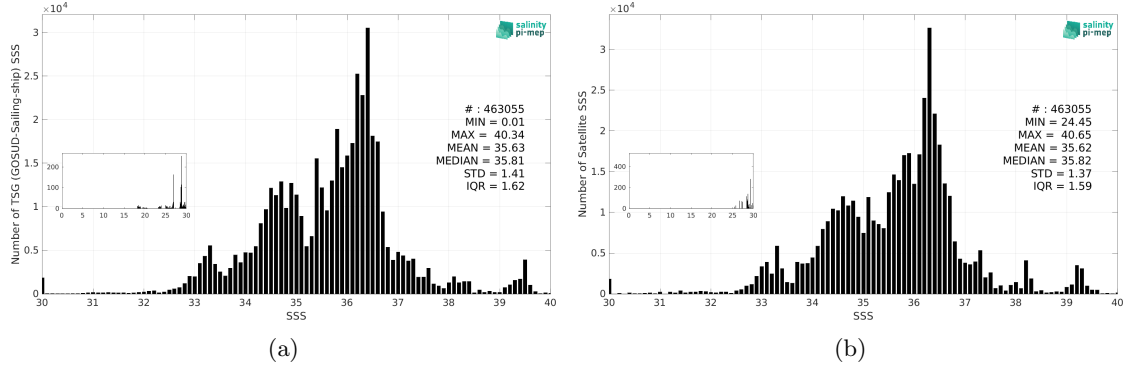
Figure 3: Histograms of SSS from TSG (GOSUD-Sailing-ship) (a) and CCI SSS L4 Merged-OI v4.41 - 7-day running (ESA) (b) considering all match-up pairs per bins of 0.1 over the Mid-Low Latitudes 45N-45S Pi-MEP region and for the full satellite product period.
