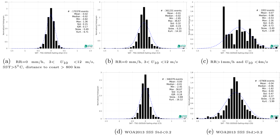
Figure 15: Normalized histogram of \Delta SSS (CCI SSS L4 Merged-OI v4.41 - 7-day running (ESA) - TSG (GOSUD-Sailing-ship)) for 5 different subdatasets corresponding to: RR=0 mm/h, 3 < U_{10} < 12 m/s, SST>5°C, distance to coast > 800 km (a), RR=0 mm/h, 3 < U_{10} < 12 m/s (b), RR>1mm/h and U_{10} < 4 m/s (c), WOA2013 SSS Std<0.2 (d), WOA2013 SSS Std>0.2 (e).
