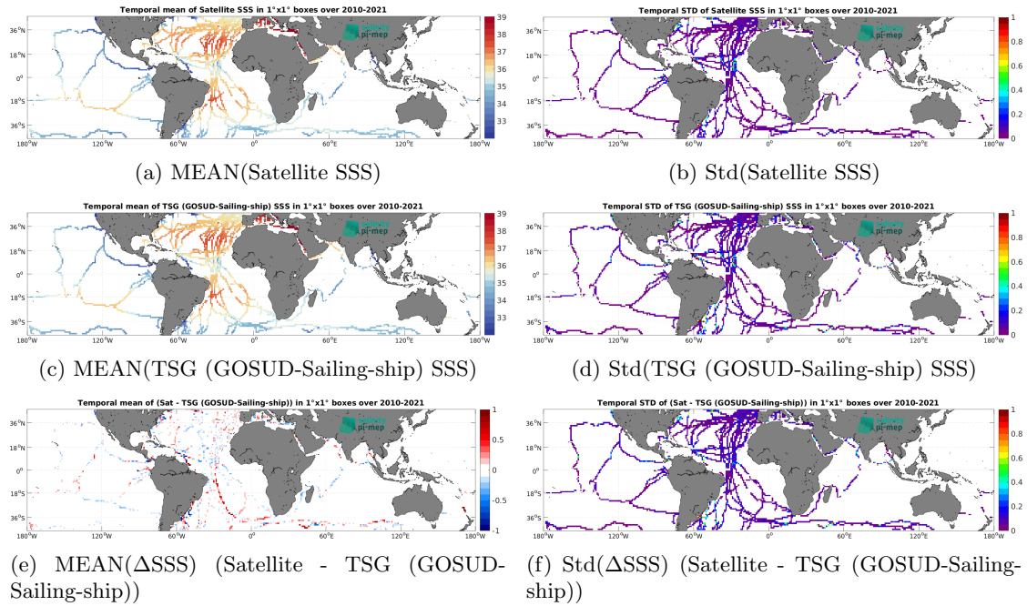
Figure 7: Temporal mean (left) and Std (right) of SSS from CCI SSS L4 Merged-OI v4.41 - 7-day running (ESA) (top), TSG (GOSUD-Sailing-ship) (middle), and of \Delta SSS (Satellite - TSG (GOSUD-Sailing-ship)). Only match-up pairs are used to generate these maps.
