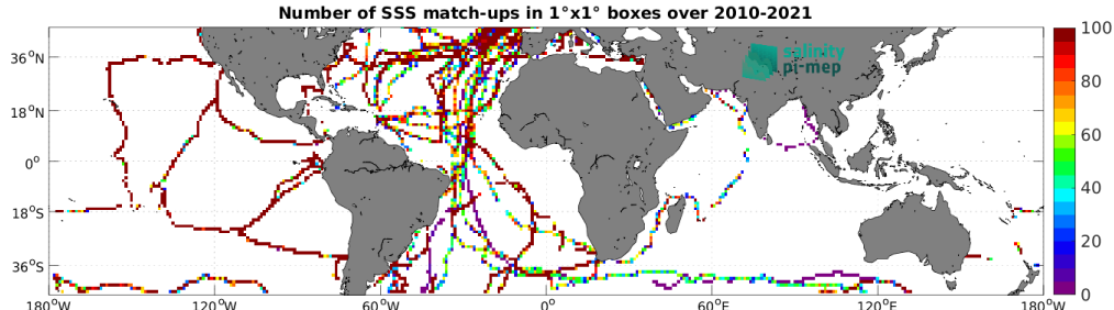
Figure 5: Number of SSS match-ups between TSG (GOSUD-Sailing-ship) SSS and the CCI SSS L4 Merged-OI v4.41 - 7-day running (ESA) SSS product for the Mid-Low Latitudes 45N-45S Pi-MEP region over 1^{\circ} \times 1^{\circ} boxes and for the full satellite product period.
