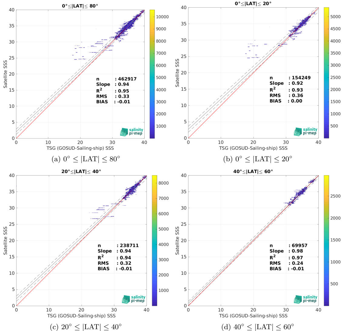
Figure 10: Contour maps of the concentration of CCI SSS L4 Merged-OI v4.41 - 7-day running (ESA) SSS (y-axis) versus TSG (GOSUD-Sailing-ship) SSS (x-axis) at match-up pairs for different latitude bands. For each plot, the red line shows x=y . The black thin and dashed lines indicate a linear fit through the data cloud and the \pm 95\% confidence levels, respectively. The number match-up pairs n , the slope and R^2 coefficient of the linear fit, the root mean square (RMS) and the mean bias between satellite and in situ data are indicated for each latitude band in each plots.
