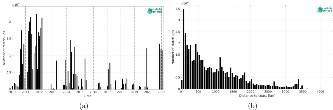
Figure 2: Number of match-ups between TSG (GOSUD-Sailing-ship) and CCI SSS L4 Merged-OI v4.41 - 7-day running (ESA) SSS as a function of time (a) and as function of the distance to coast (b) over the Mid-Low Latitudes 45N-45S Pi-MEP region and for the full satellite product period.
