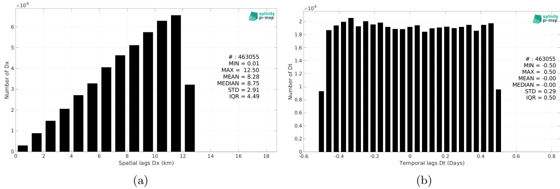
Figure 6: Histograms of the spatial (a) and temporal (b) lags between the location/time of the TSG (GOSUD-Sailing-ship) measurement and the date of the corresponding CCI SSS L4 Merged-OI v4.41 - 7-day running (ESA) SSS pixel.
