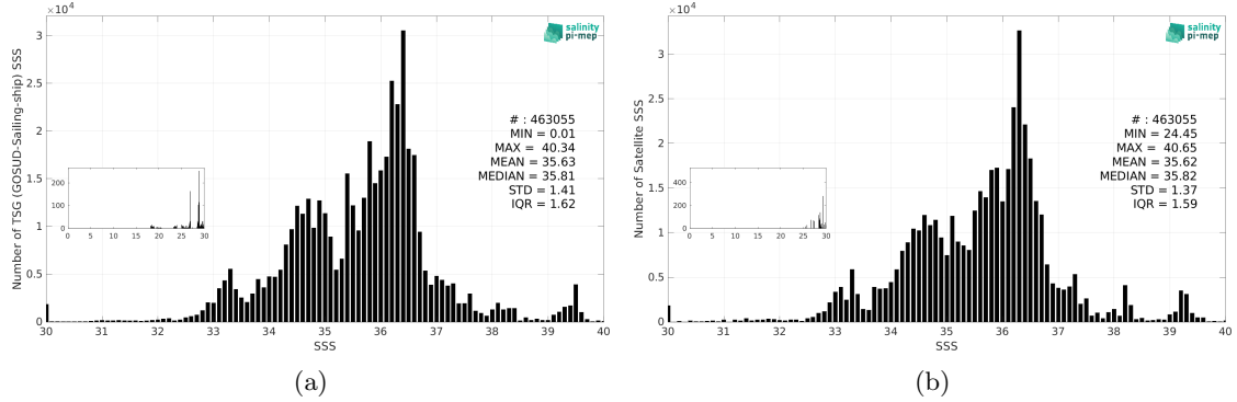
Figure 3: Histograms of SSS from TSG (GOSUD-Sailing-ship) (a) and CCI SSS L4 Merged-OI v4.41 - 7-day running (ESA) (b) considering all match-up pairs per bins of 0.1 over the Mid-Low Latitudes 45N-45S Pi-MEP region and for the full satellite product period.
